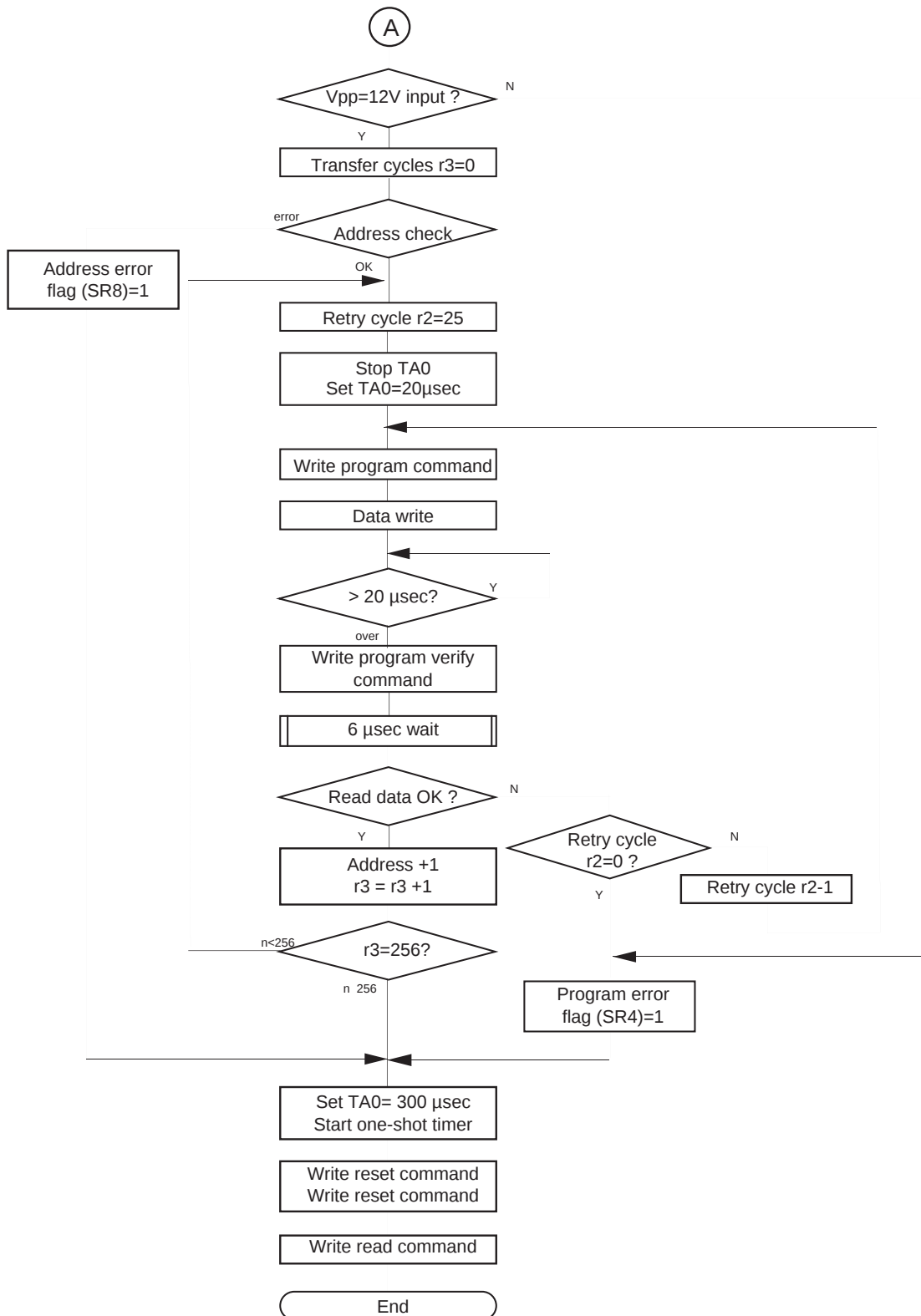
Figure 2.2.11 Page Program (2)
