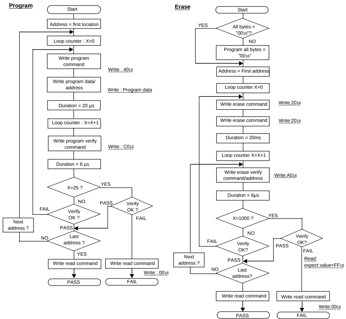
Figure 2.1.3 Program and Erase Execution Flowchart in The CPU Rewrite Mode
