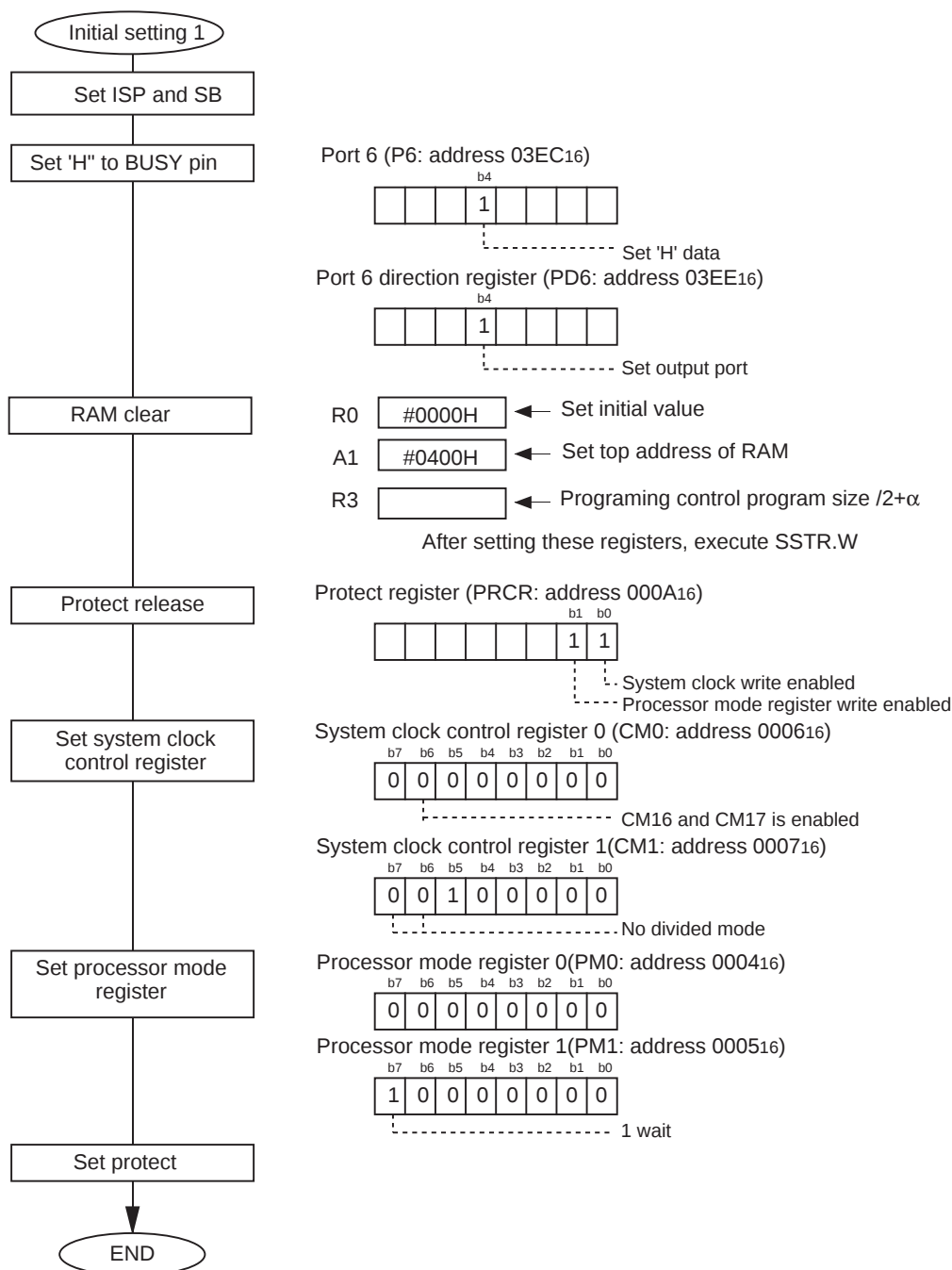
Figure 3.2.3 Initialization 1
