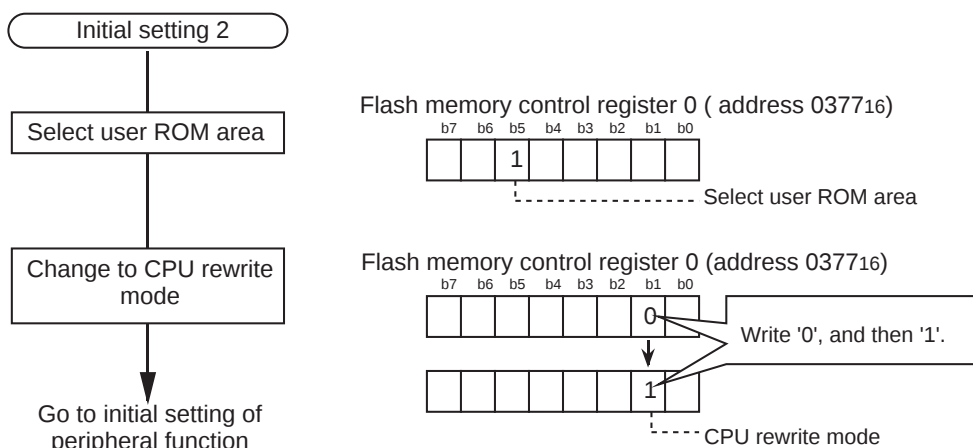
Figure 4.2.5 Initialization 2
