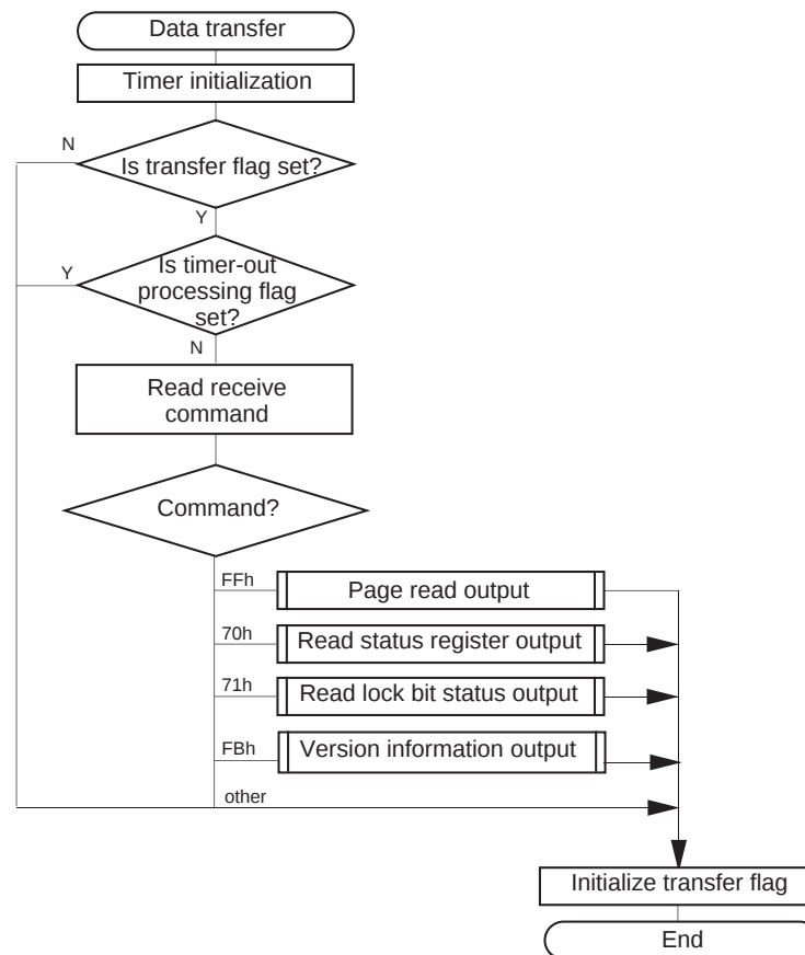
Figure 4.2.22 Data Transfer
