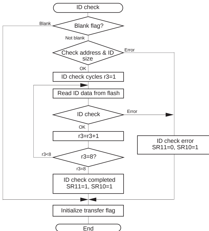
Figure 3.2.20 ID Check
