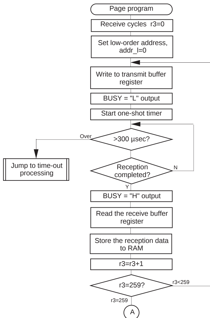
Figure 2.2.10 Page Program (1)
