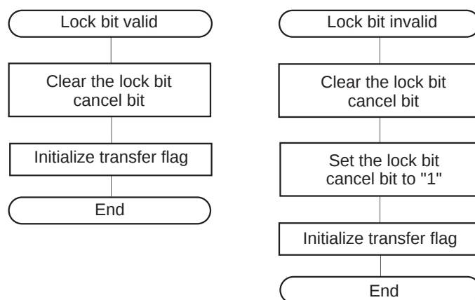
Figure 4.2.19 Lock Bit Enable/Disable
