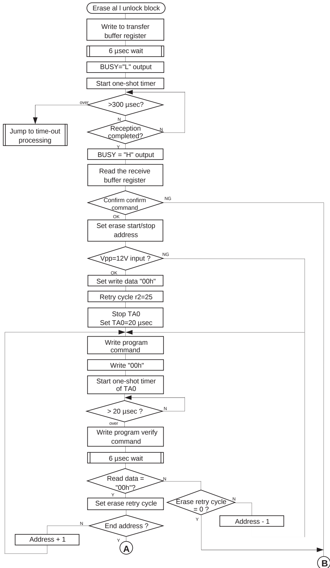
Figure 2.2.12 Erase All Unlock Block (1)
