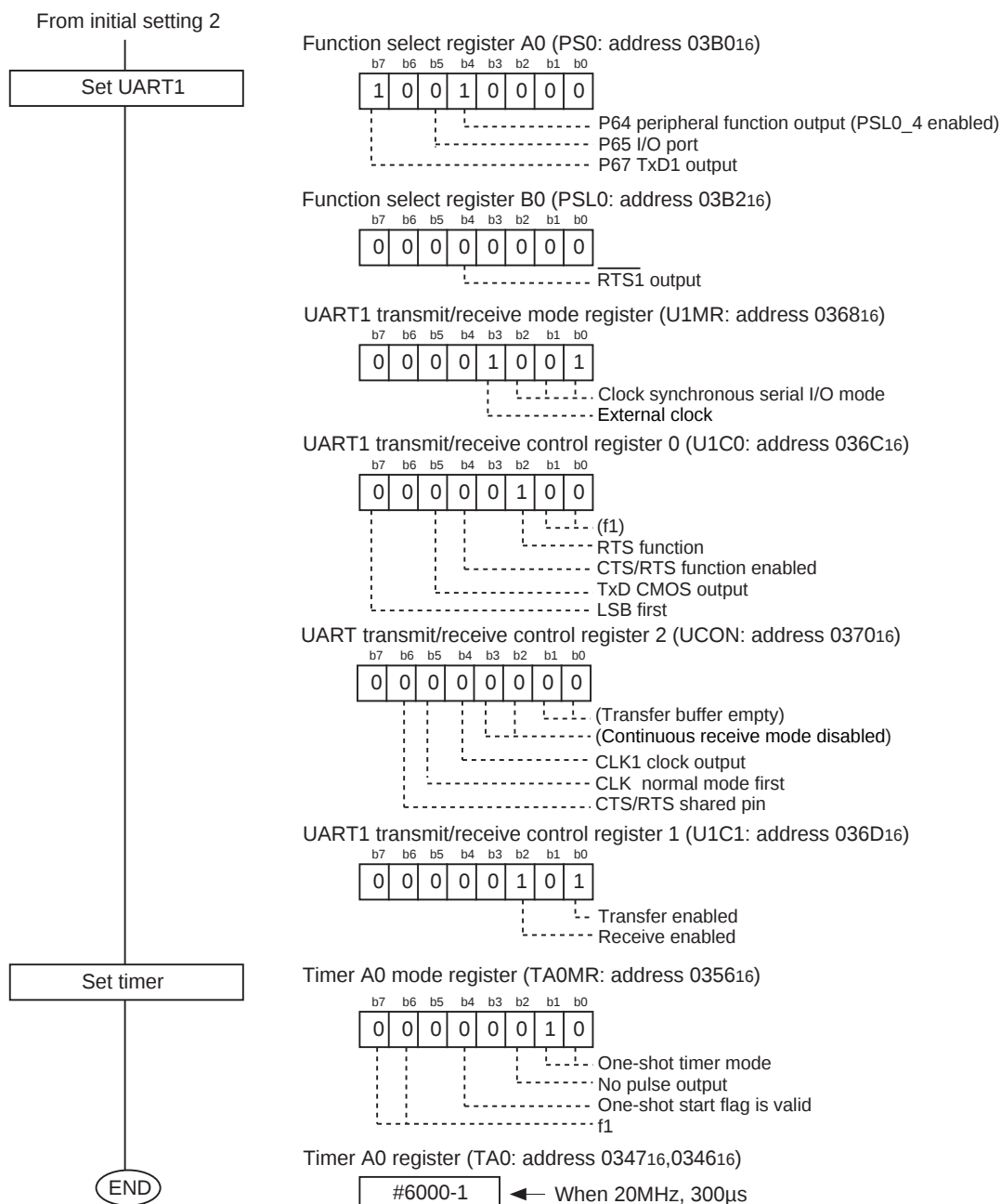
Figure 4.2.6 Initialization 2 (Peripheral Function)
