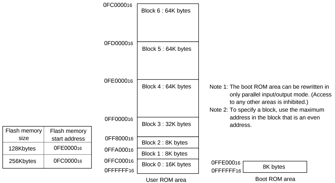
Figure 4.1.1 Memory Map
