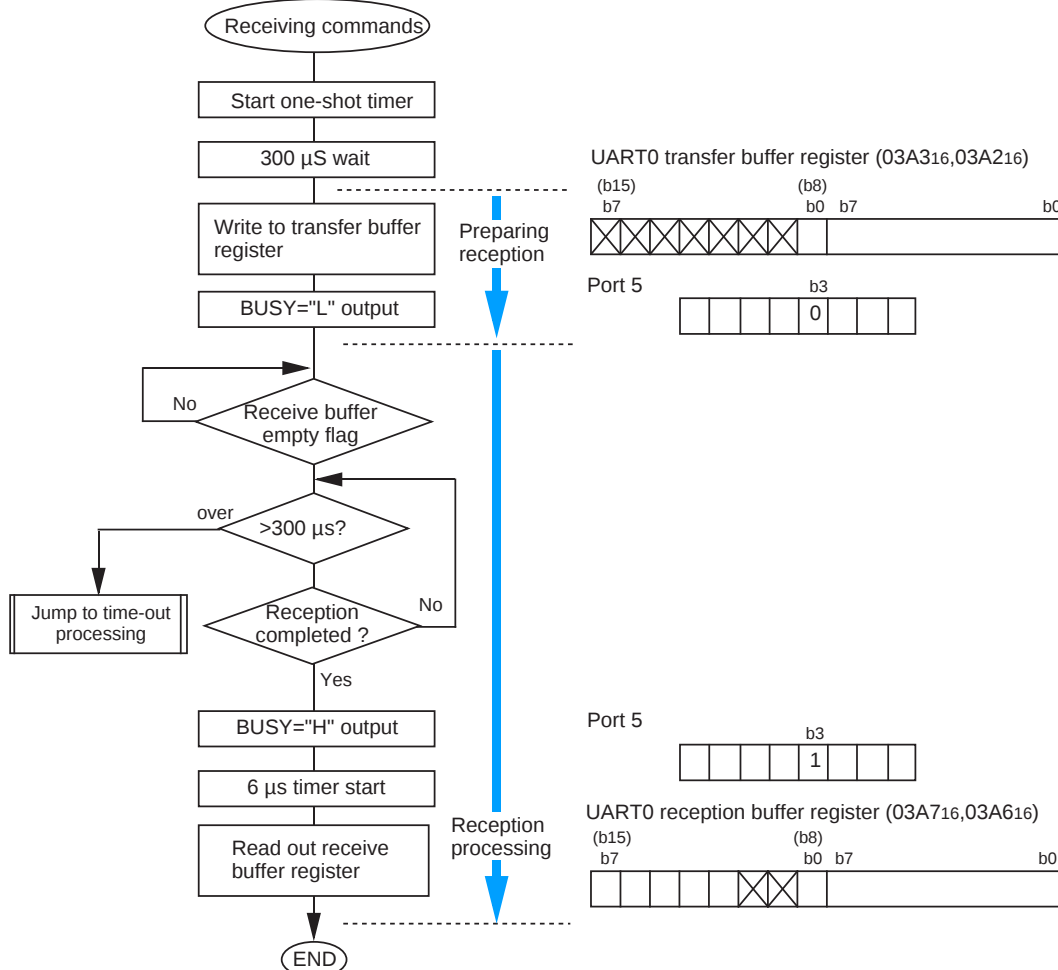
Figure 2.2.7 Receiving Commands
