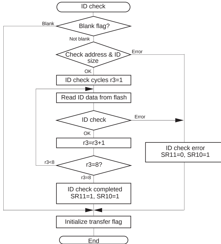
Figure 4.2.20 ID Check
