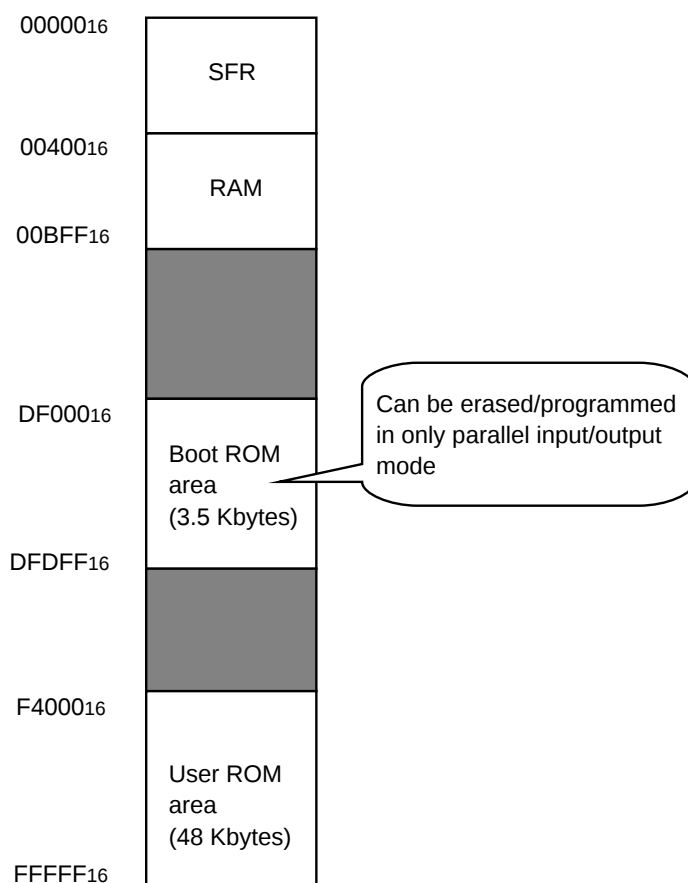
Figure 2.1.1 M30201F6 Memory Map
