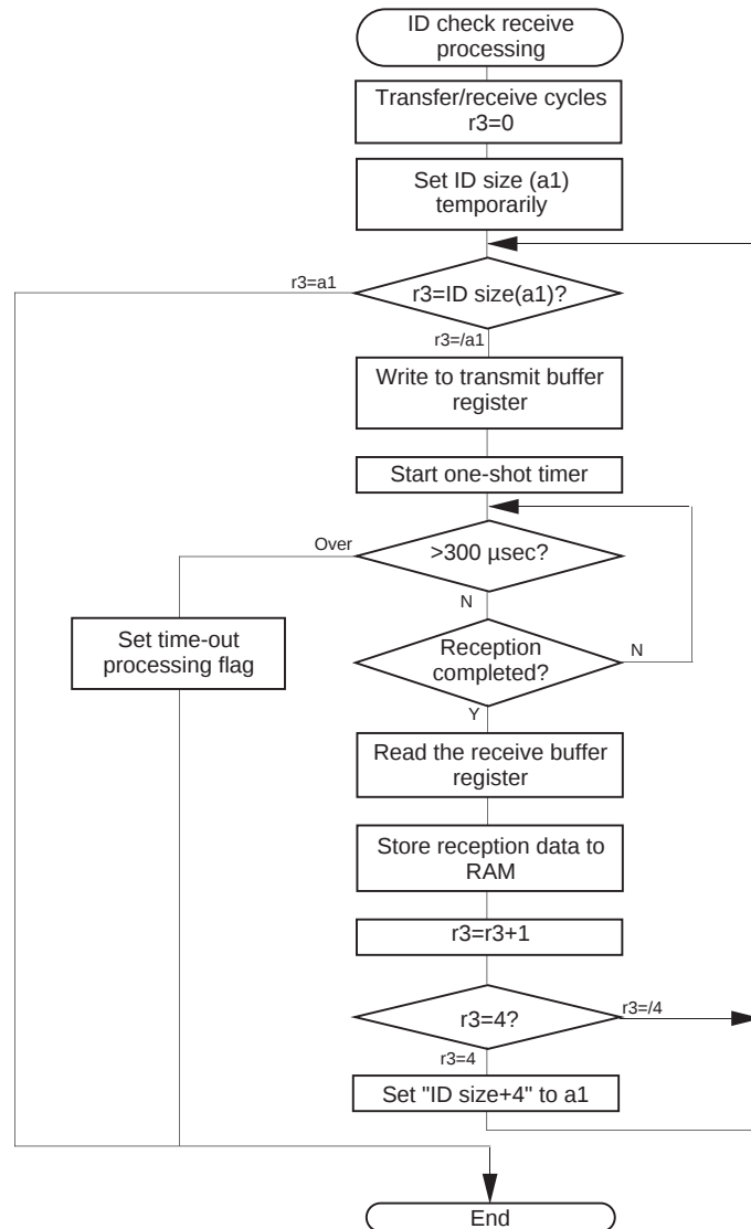
Figure 4.2.8 ID Data Receive Process
