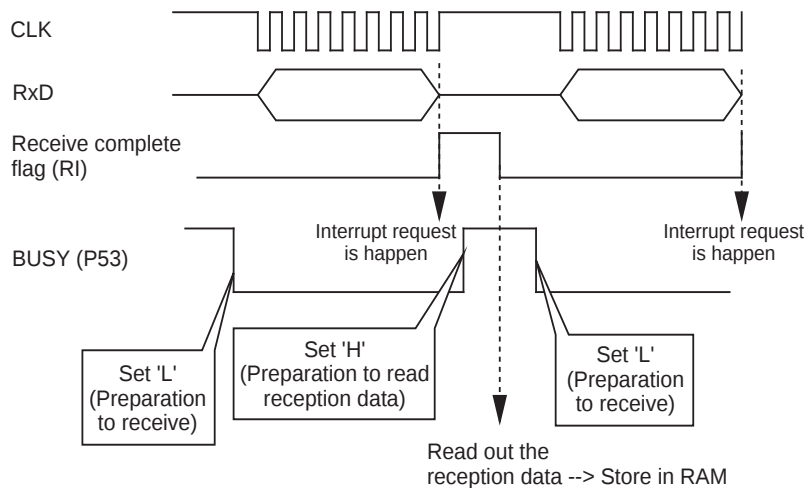
Figure 2.2.8 BUSY Signal Control Timing
