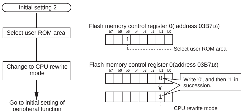
Figure 3.2.5 Initialization 2
