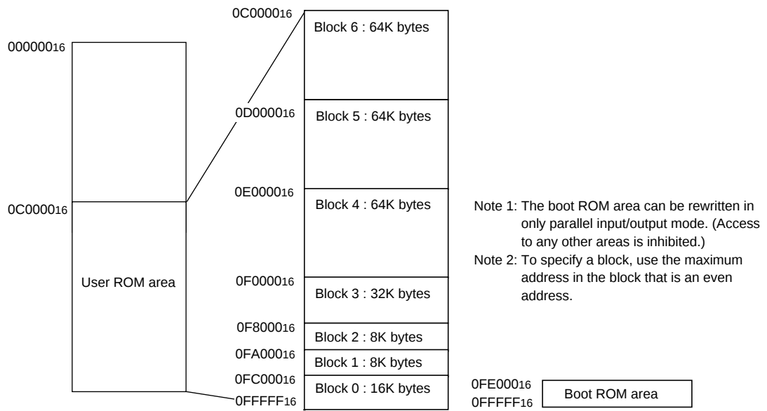
Figure 3.1.1 M30624FG memory Map
