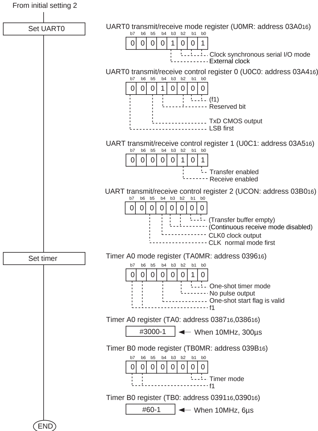
Figure 2.2.6 Initialization 2 (Peripheral Function)
