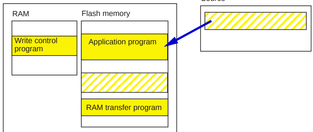
Figure 1.3.1 Operation When Controlling Flash Memory
