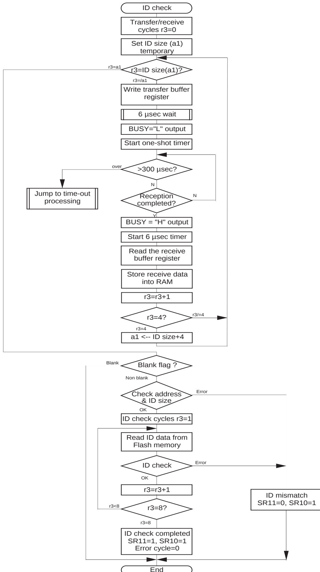
Figure 2.2.16 ID Check
