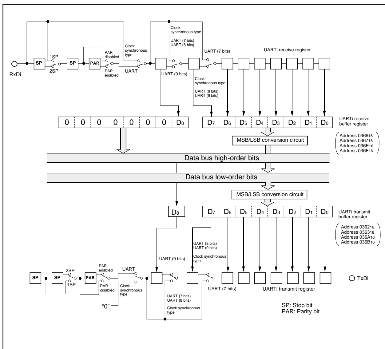
Figure 1.16.3. Block diagram of UART i (i = 0, 1) transmit/receive unit
