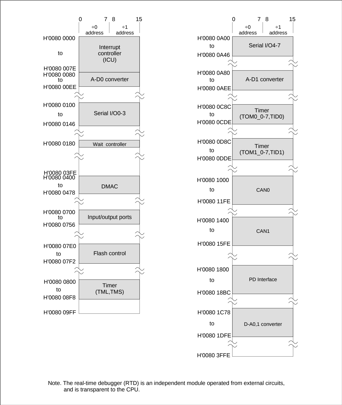
Figure 5. SFR Area
