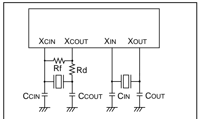
Fig. 53 Ceramic resonator circuit
