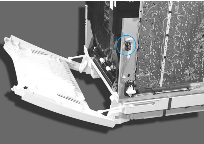
Figure 7-18 Door switch
