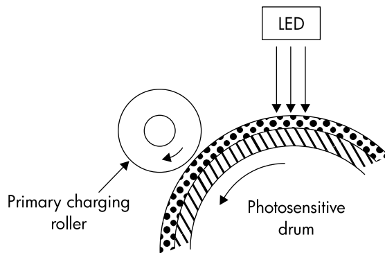
Figure 5-19 Primary exposure
