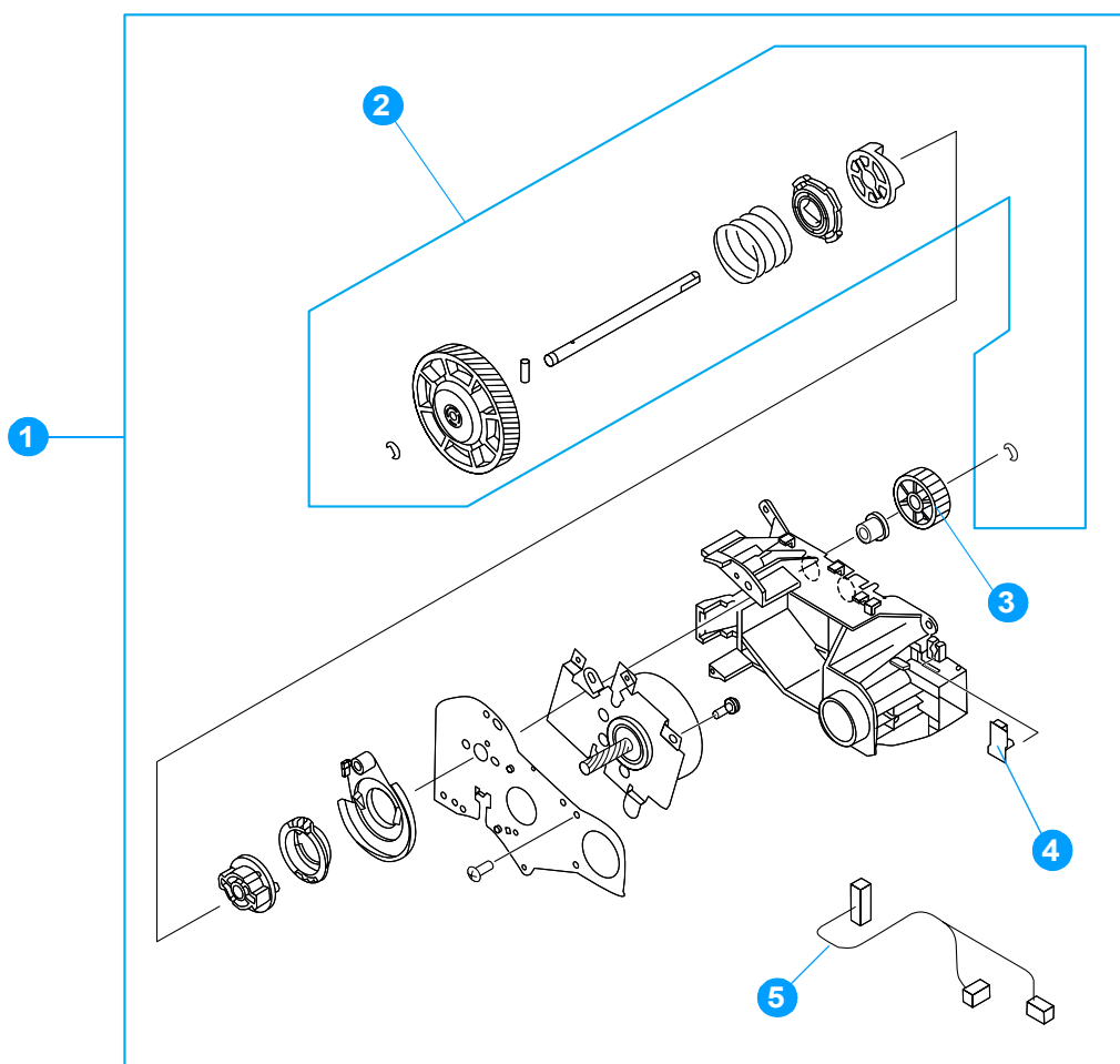
Figure 8-10 Drum drive assembly
