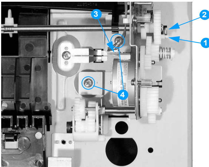
Figure 6-72 Removing and replacing the paper feeder drive unit, top view (1 of 2)
