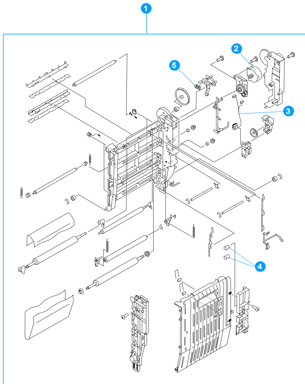
Figure 8-16 ETB assembly
