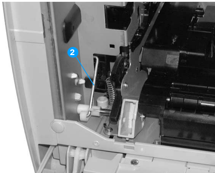
Figure 6-36 Removing and replacing the interlock arm
