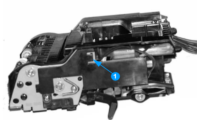
Figure 6-20 Removing and replacing the paper pickup sensor PCB (1 of 2)
