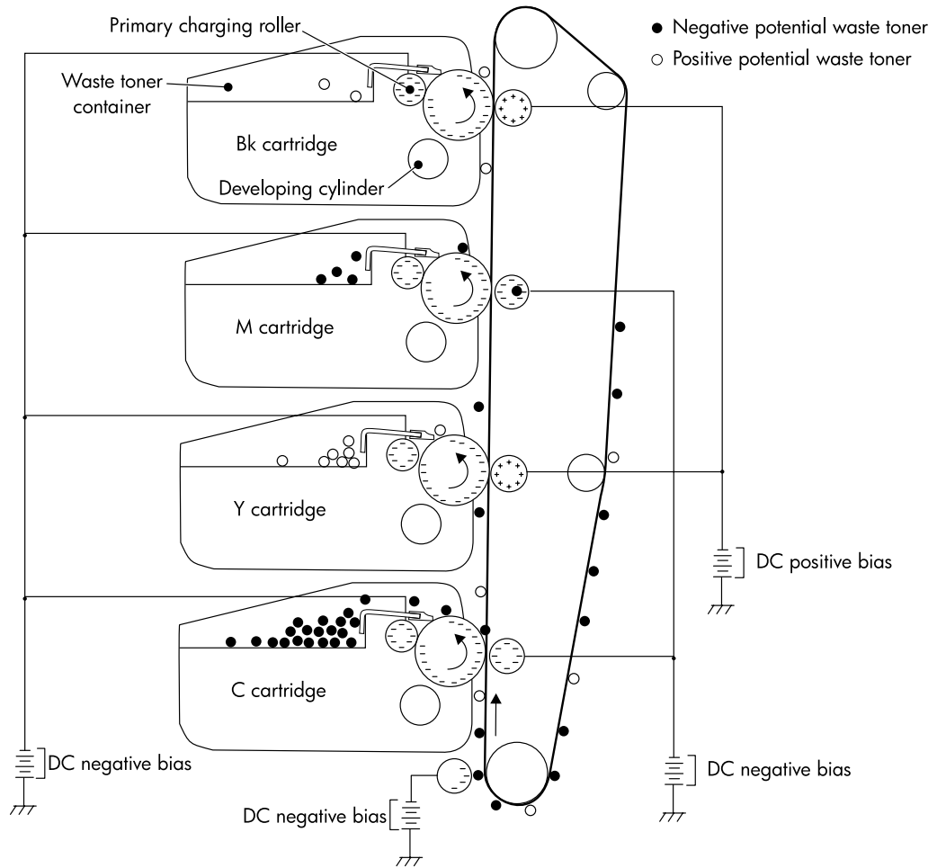
Figure 5-27 ETB cleaning
