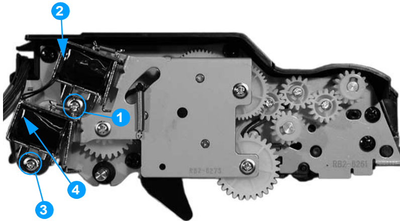
Figure 6-27 Removing and replacing the solenoids
