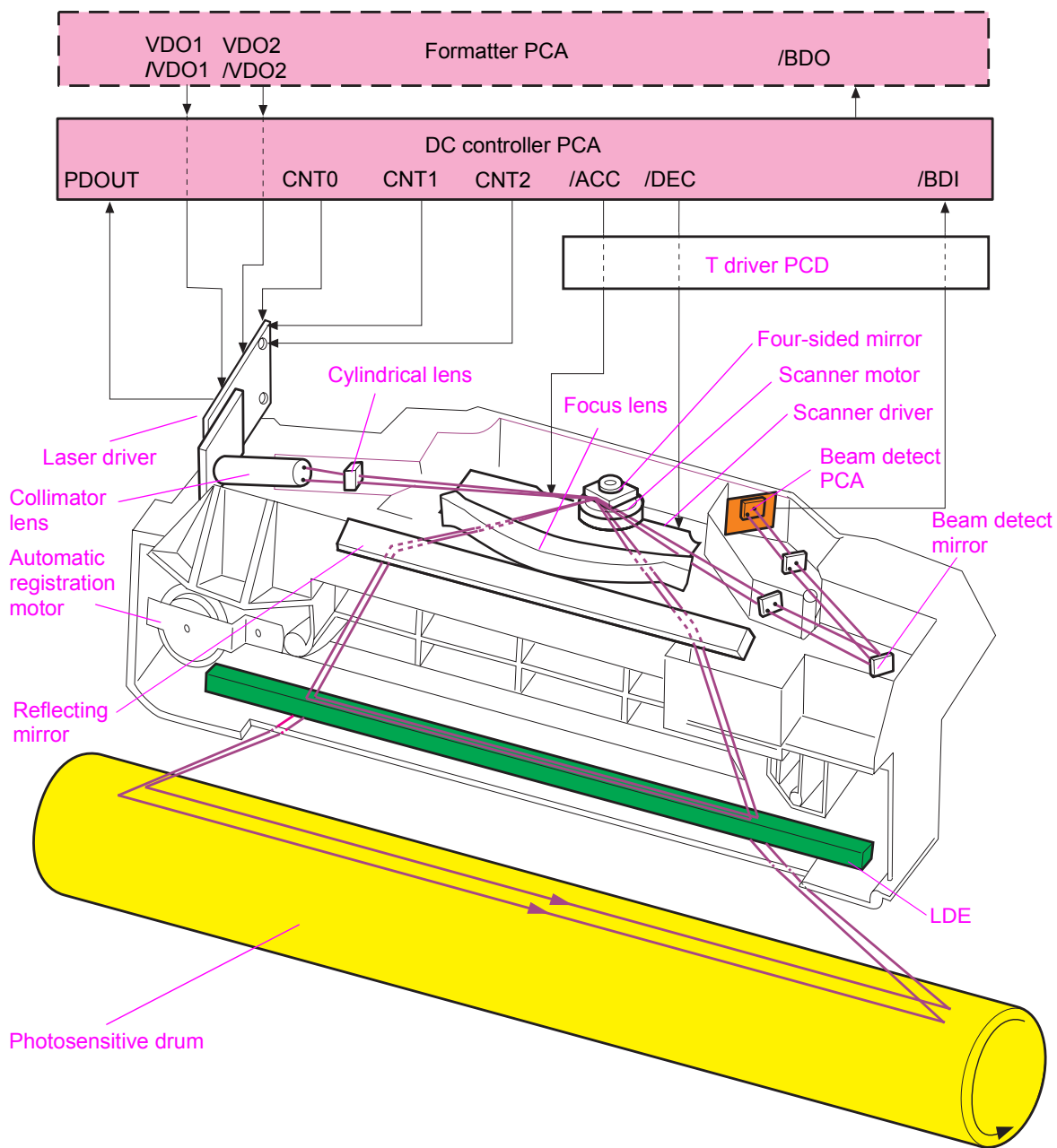
Figure 39. Laser/scanner system
