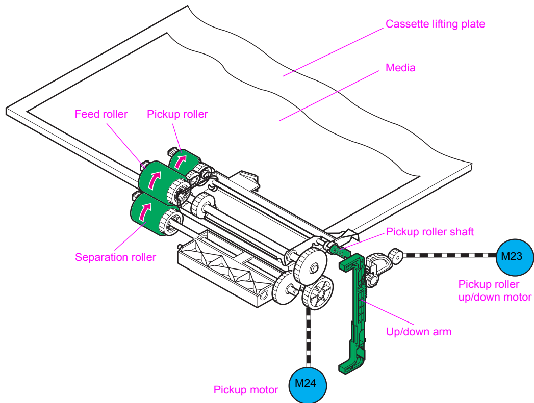
Figure 62. Cassette pickup
