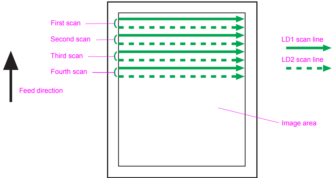
Figure 40. Dual-beam method
