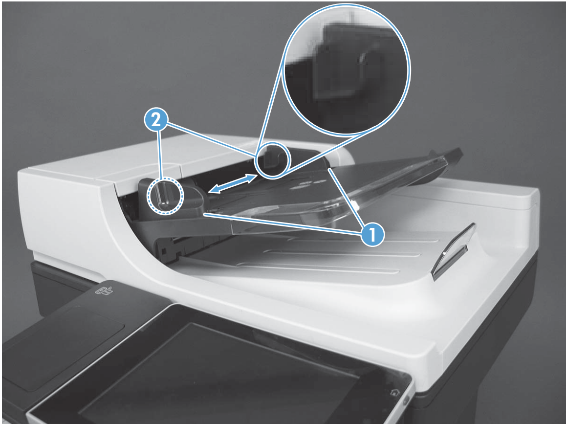
Figure 1-58 Document feeder deskew features
