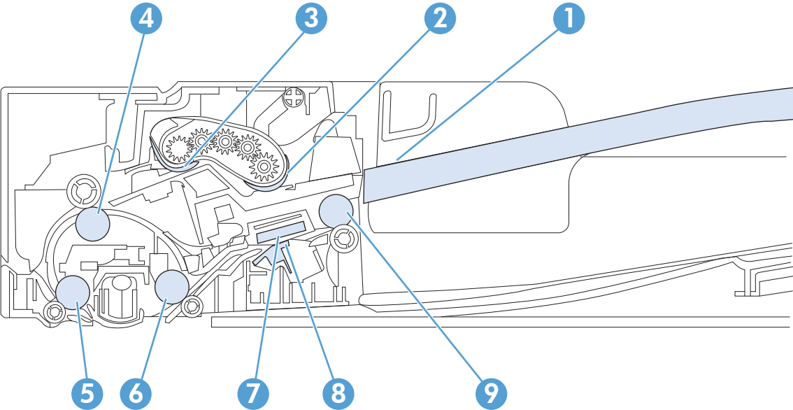
Figure 1-57 Document feeder paper path (M575c model)
