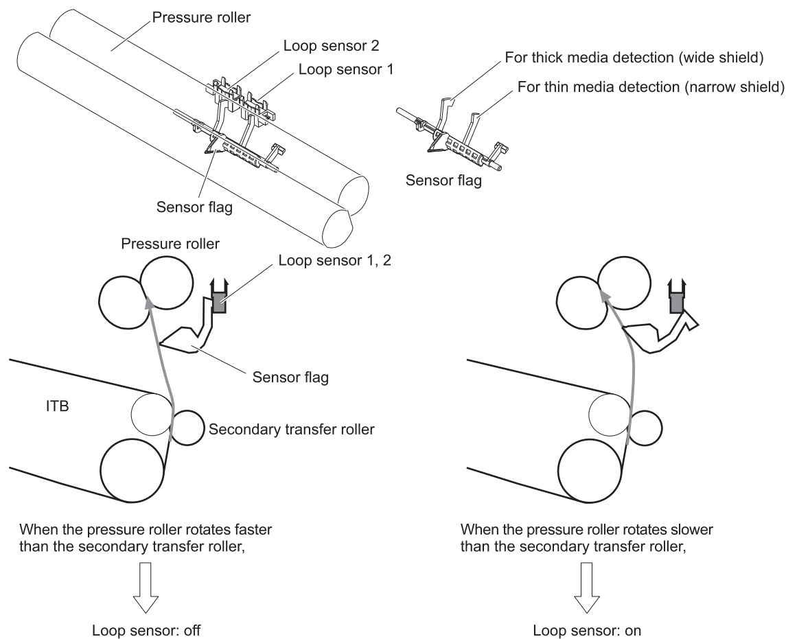
Figure 1-40 Loop-control mechanism
