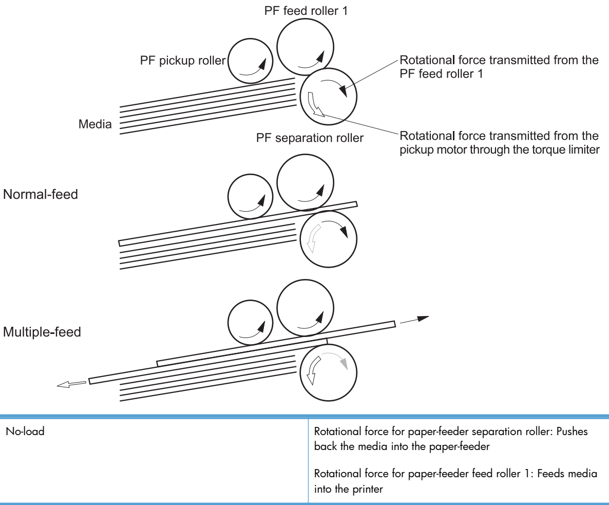
Figure 1-49 Paper-feeder multiple feed prevention
