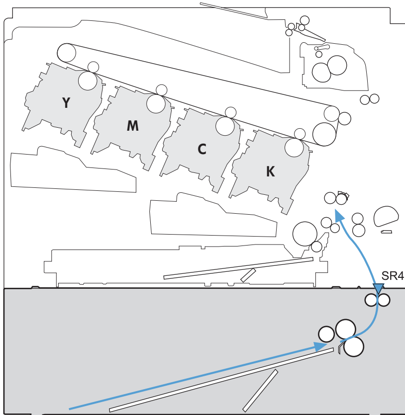
Figure 1-50 Jam detection
