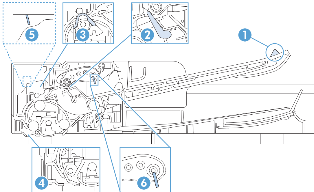
Figure 1-51 Document feeder sensors (M575dn and 575f models)
