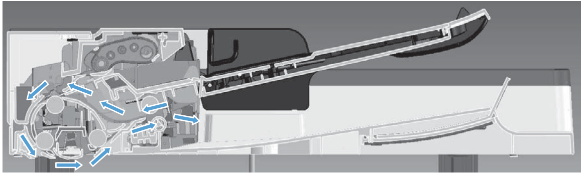
Figure 1-55 Document feeder duplex operation (M575dn and 575f models)
