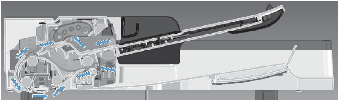
Figure 1-53 Document feeder simplex operation (M575dn and 575f models)
