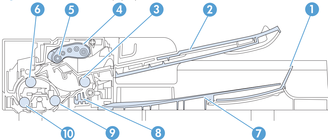
Figure 1-52 Document feeder paper path (M575dn and 575f models)
