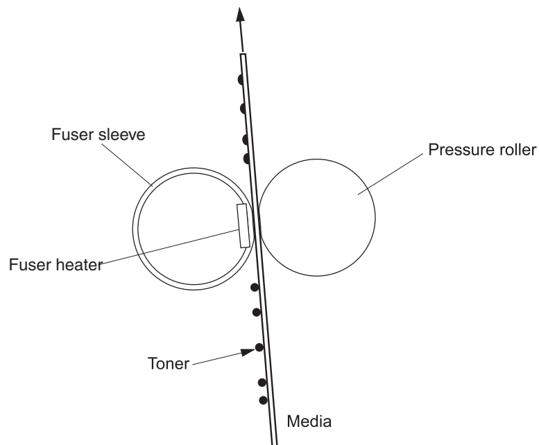
Figure 1-18 Fusing
