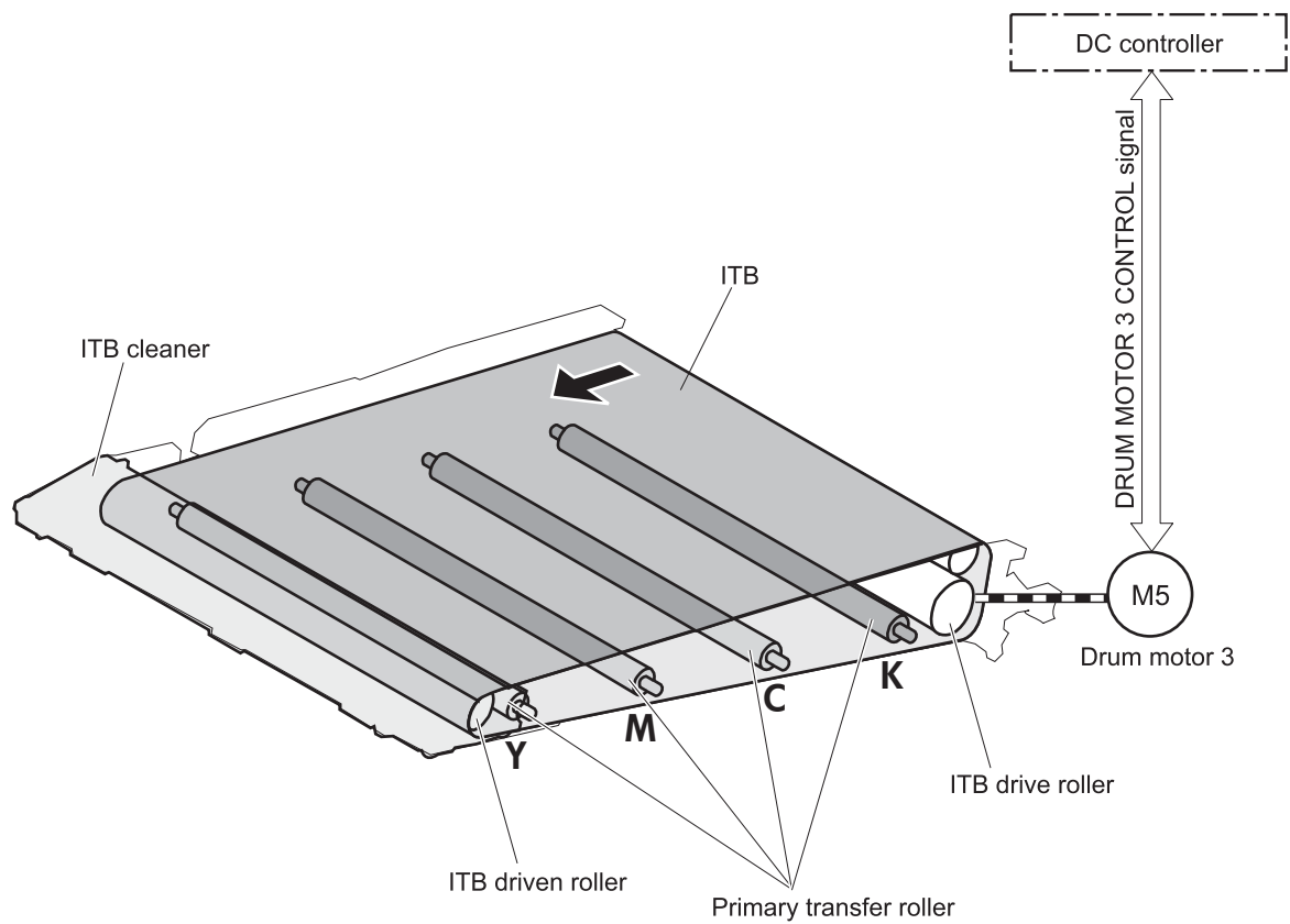
Figure 1-23 ITB unit
