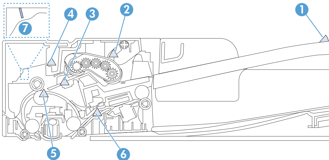
Figure 1-56 Document feeder sensors (M575c model)
