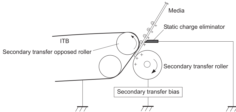
Figure 1-17 Separation
