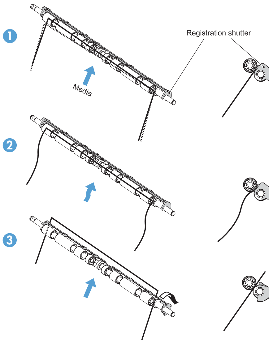
Figure 1-38 Skew-feed prevention
