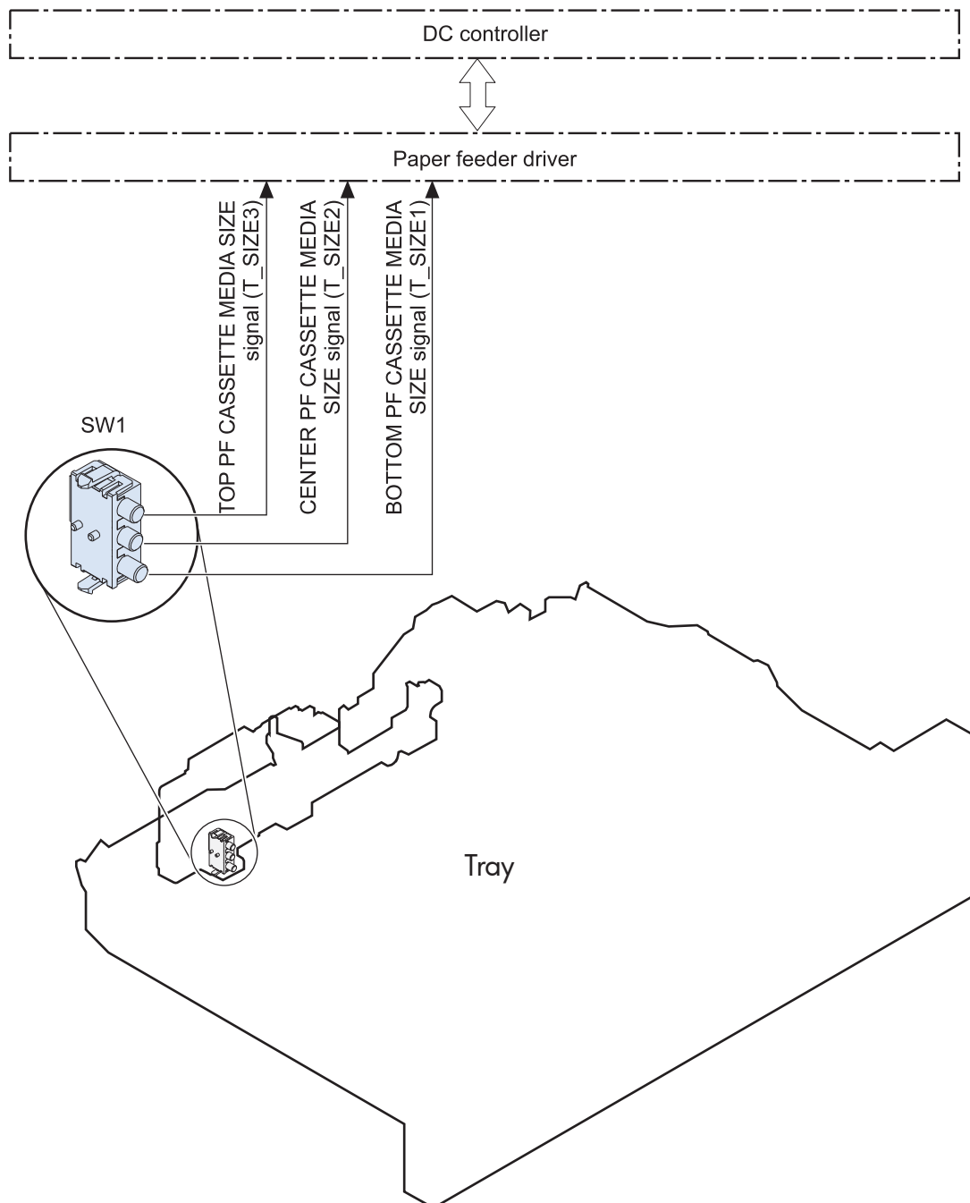
Figure 1-47 Paper size detection
