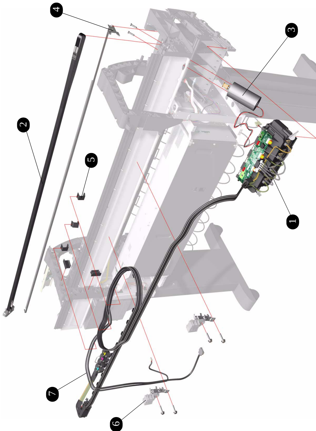
Figure 9: Scan-Axis Assemblies
