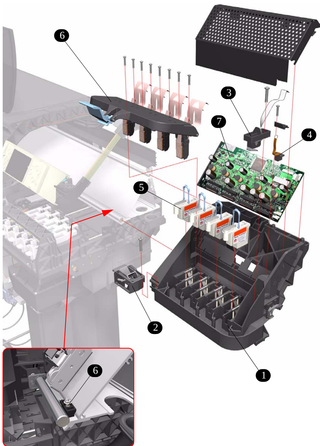
Figure 8: Carriage Assembly
