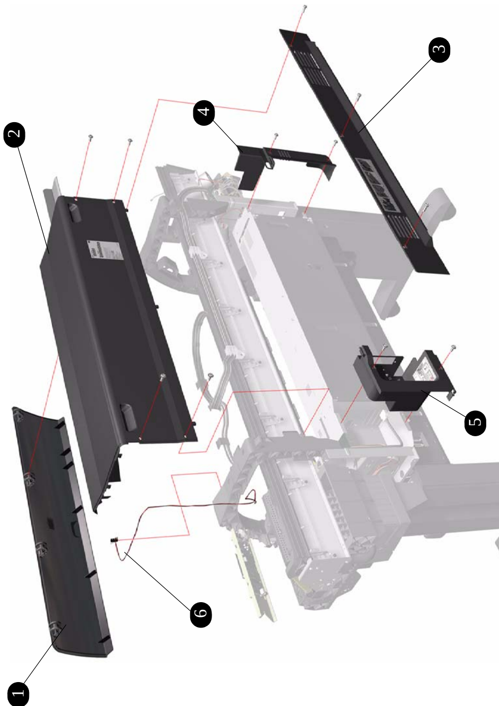
Figure 2: Center Covers
