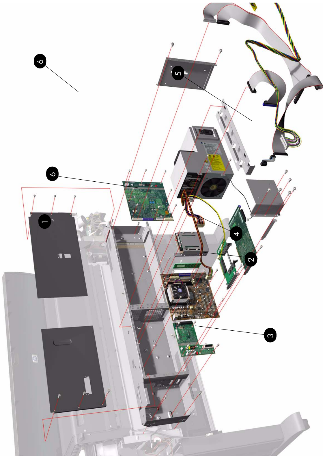
Figure 7: Electronics Module
