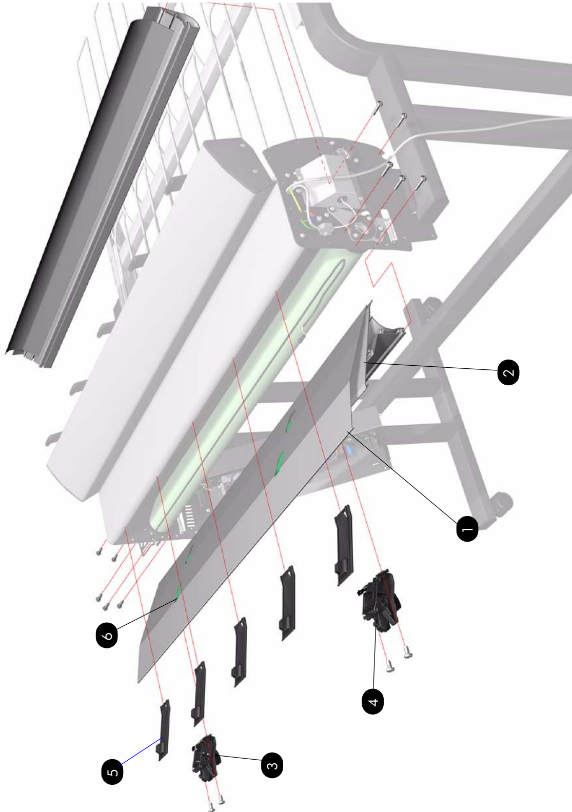
Figure 8: Input Trays
