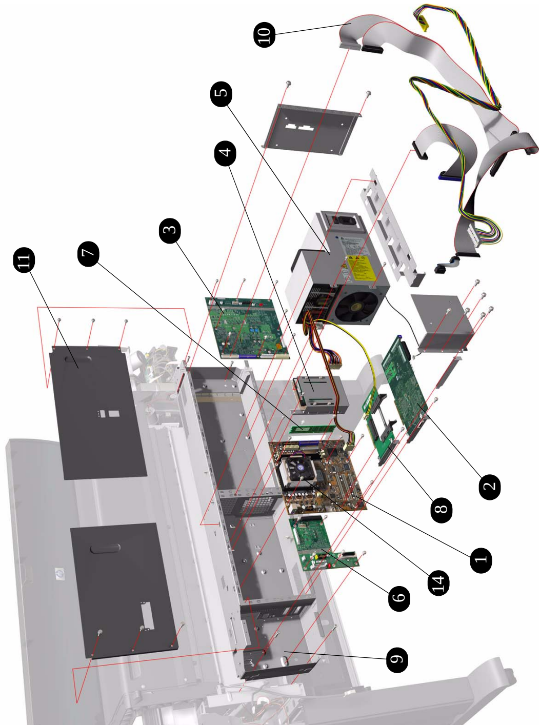
Figure 3: Electronics Module
