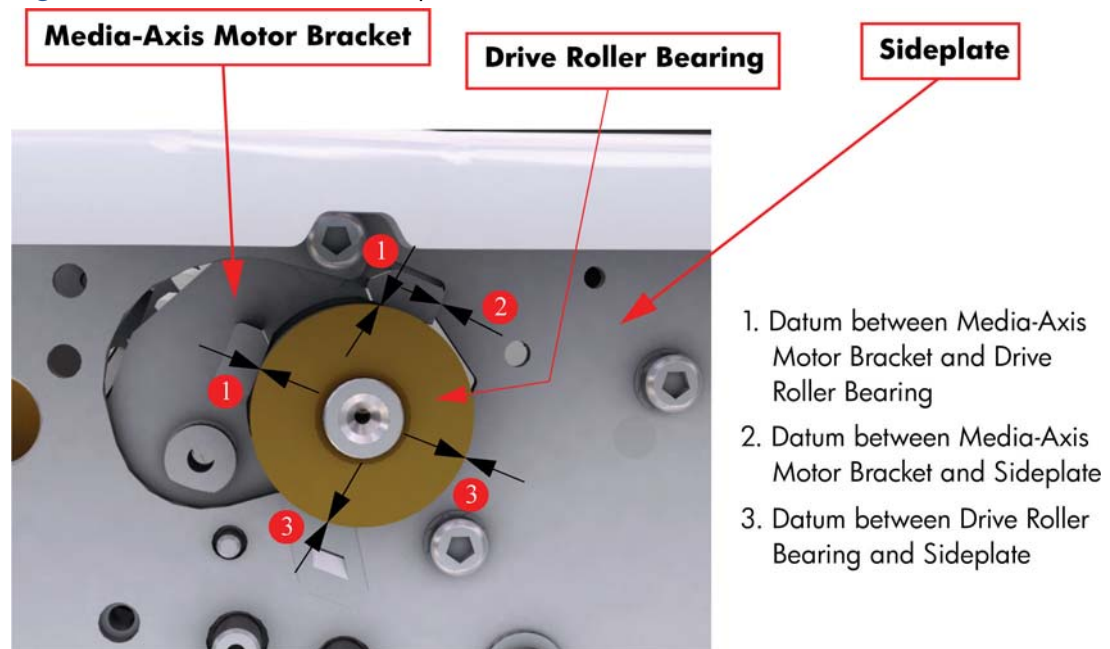
Figure 9-1 Left-Hand Side of the printer
