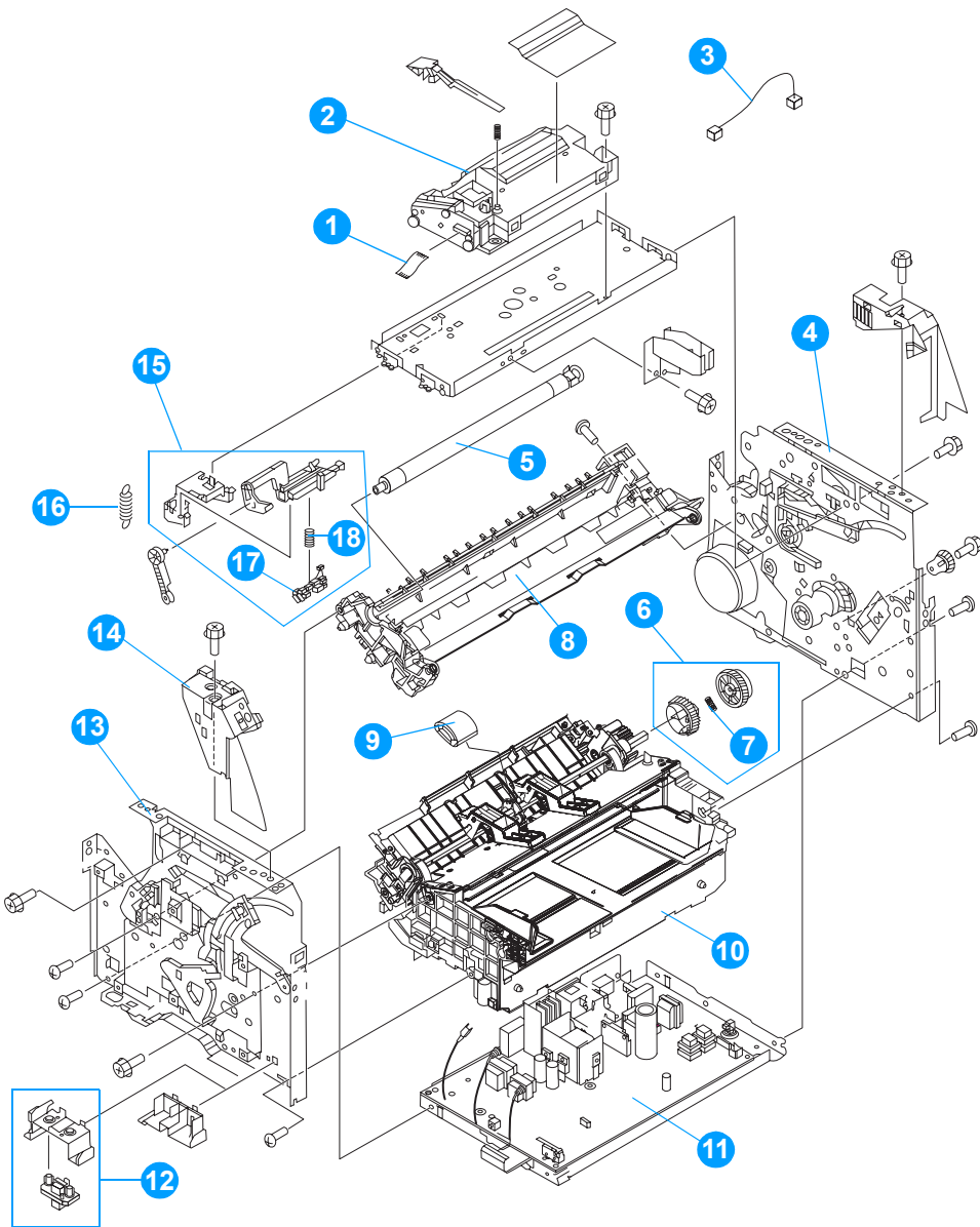
Figure 97. Internal components (1 of 2)
