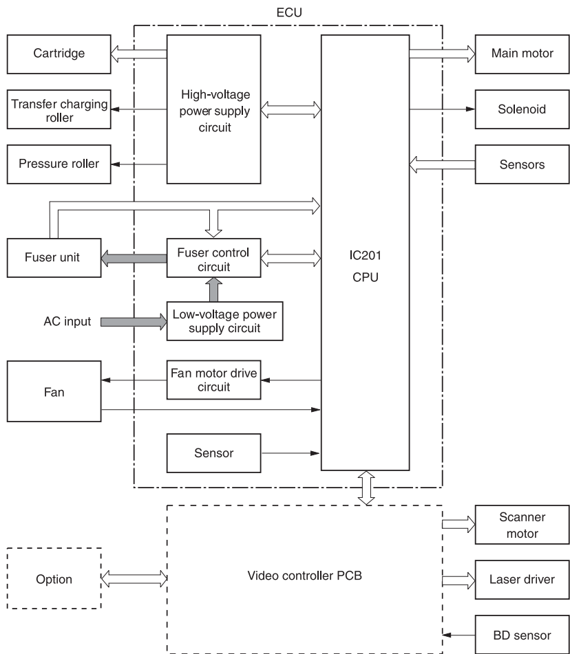
Figure 13. ECU loads
