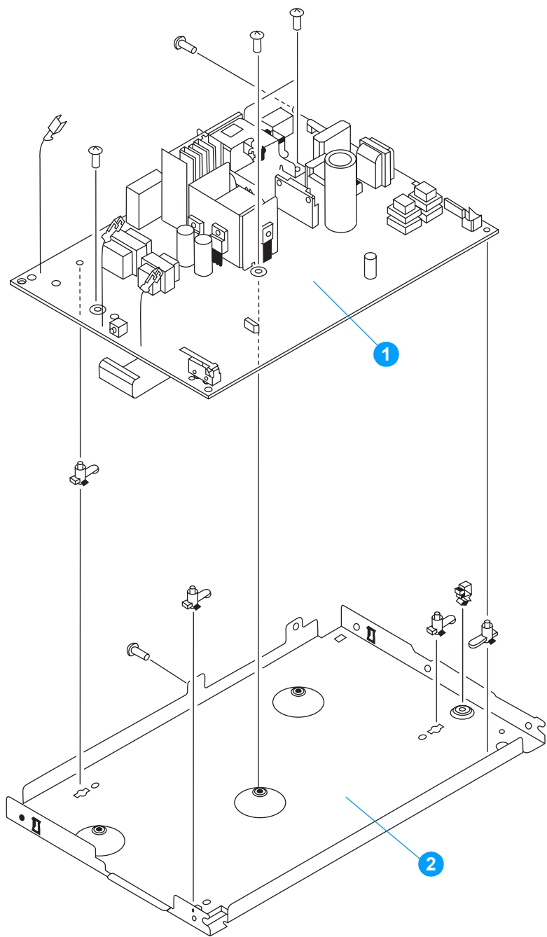
Figure 101. Electrical components
