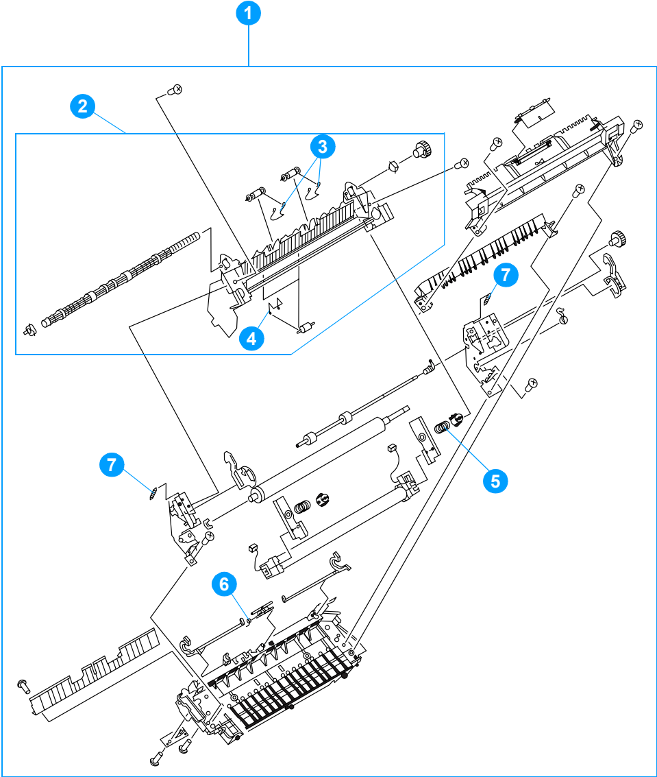
Figure 104. Fuser assembly
