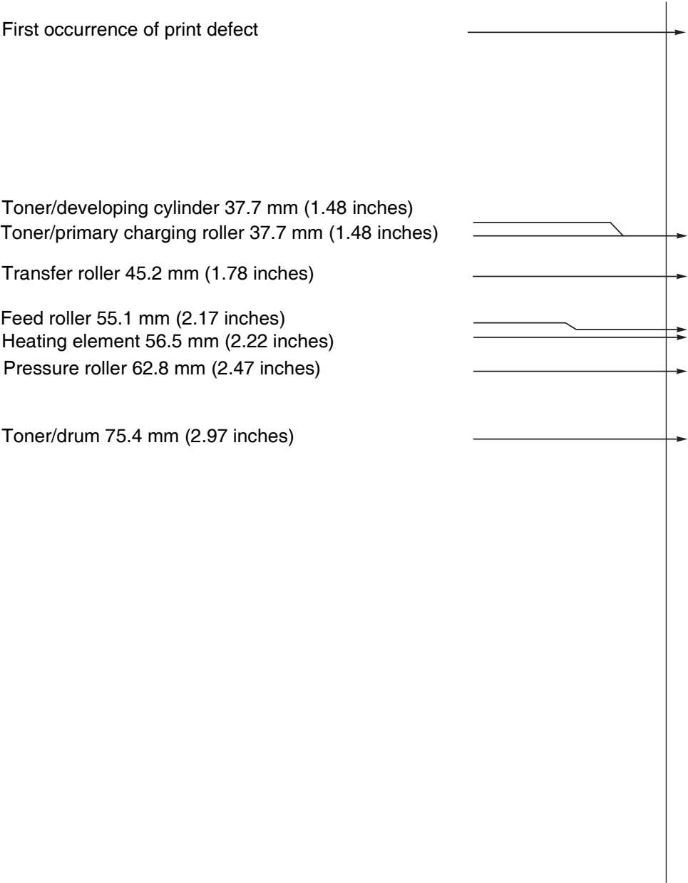
Figure 89. Repetitive image defect ruler
