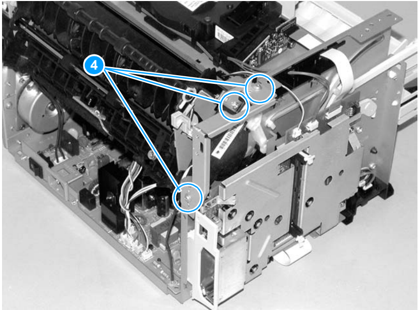
Figure 47. Removing the fuser assembly (2 of 4)
