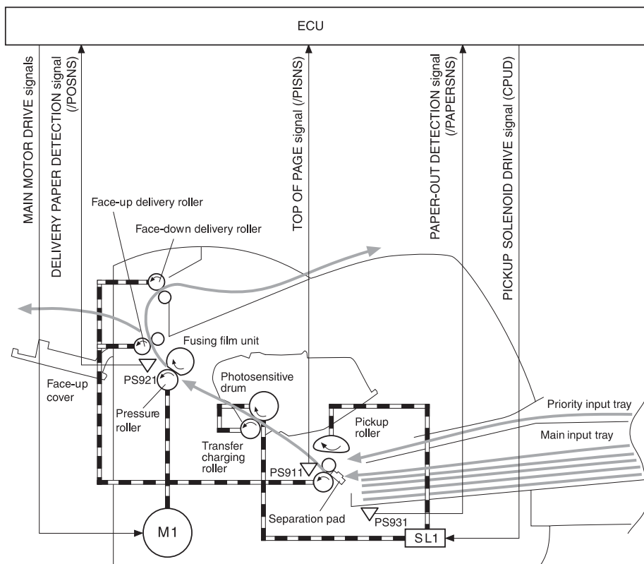
Figure 17. Printer path
