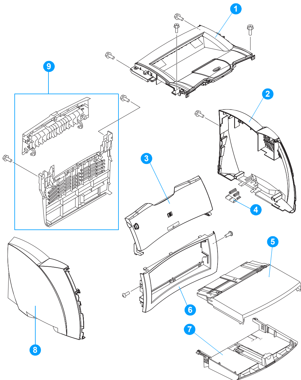
Figure 96. Covers
