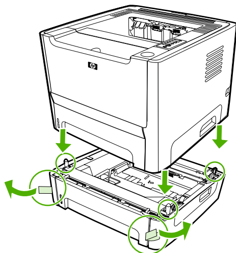
Figure 2-2 Installing tray 3
