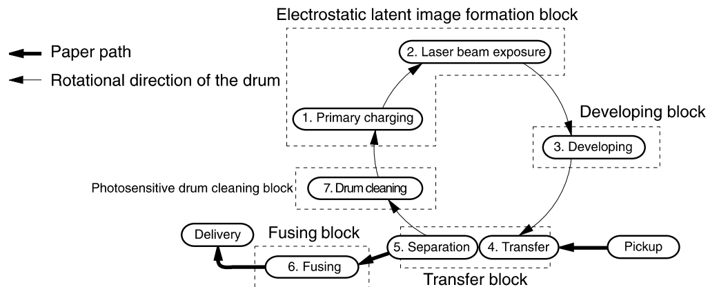
Figure 5-7 Image-formation system
