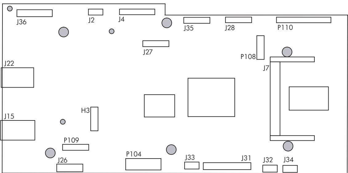
Figure 7-2 Formatter connectors
