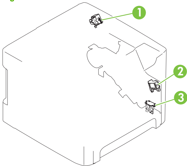
Figure 7-4 Solenoids
