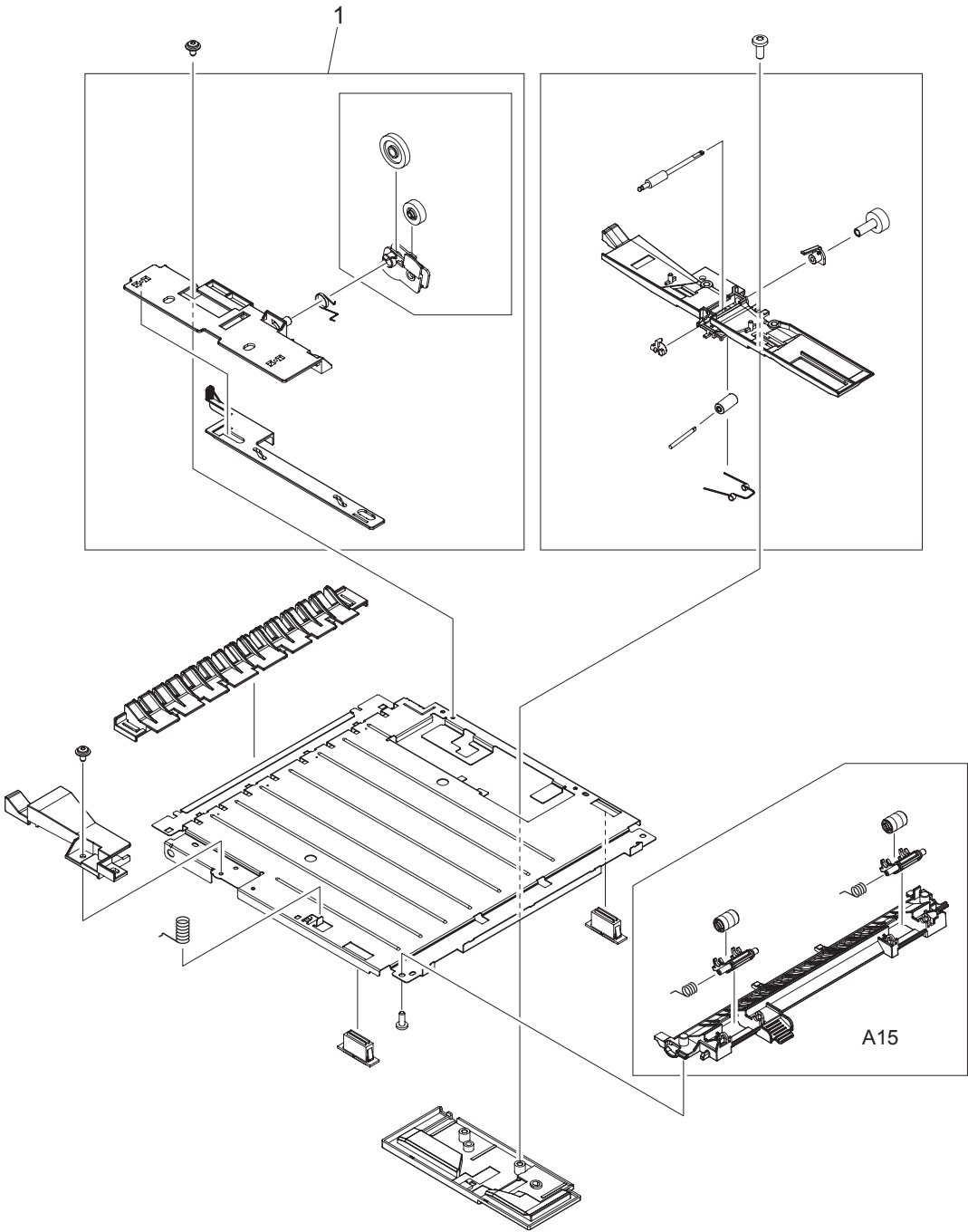
Figure 7-27 Duplexing assembly
