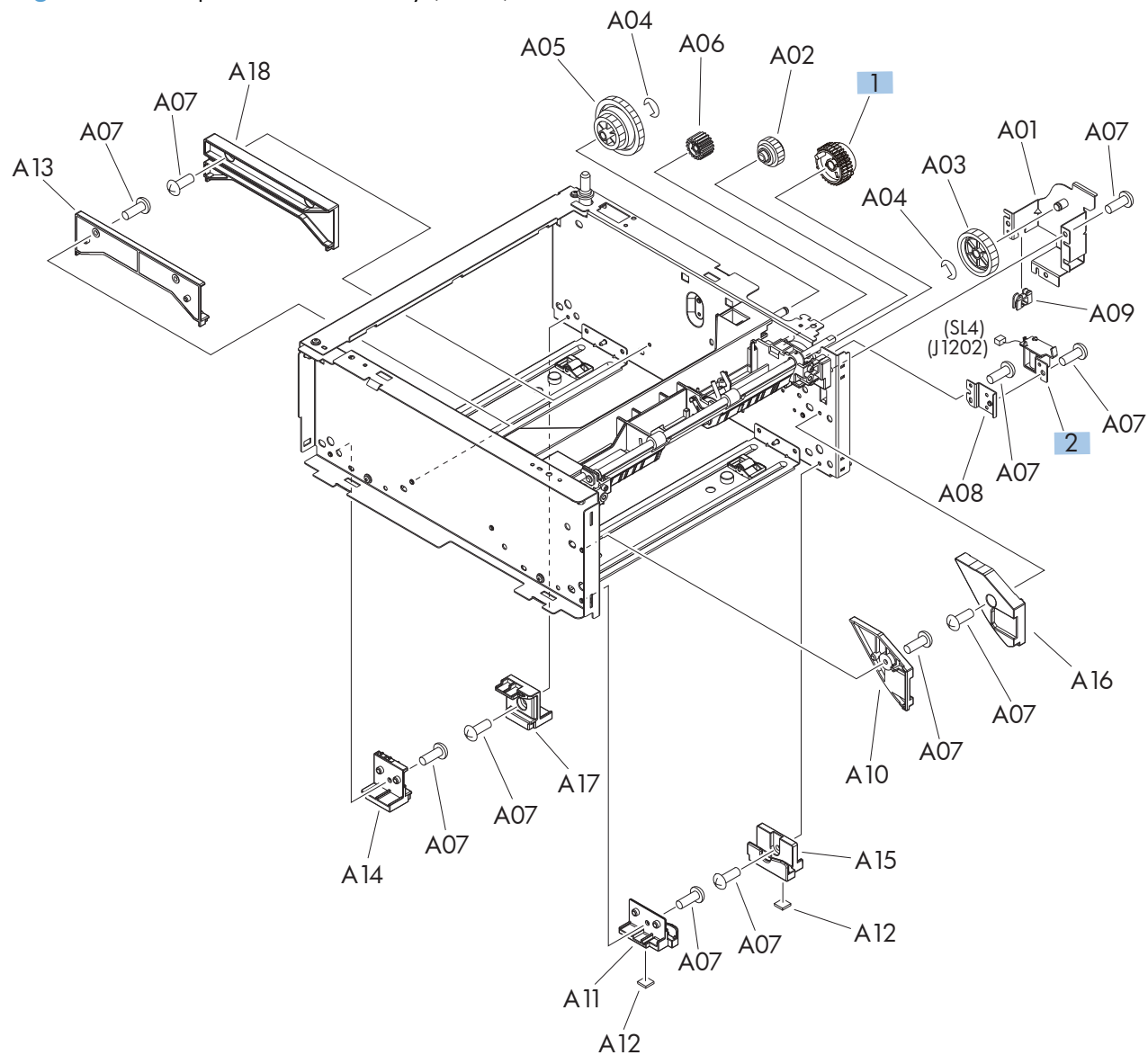
Figure 2-12 Paper feeder main body (1 of 2)
