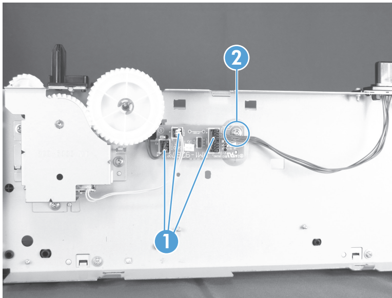
Figure 1-81 Remove the optional paper feeder driver PCA (2 of 2)
