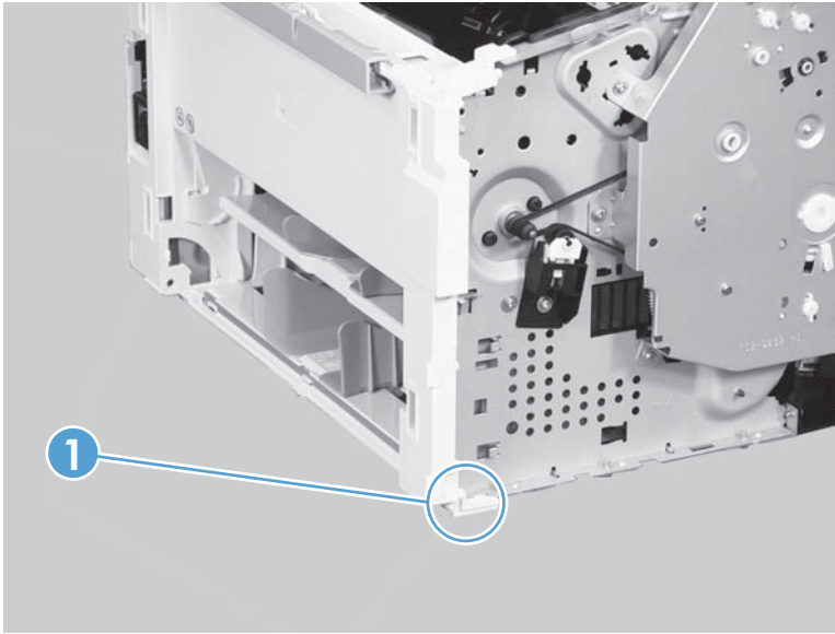
Figure 2-36 Remove the front cover (2 of 3)
