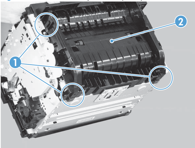
Figure 2-28 Remove the duplex frame (2 of 2)
