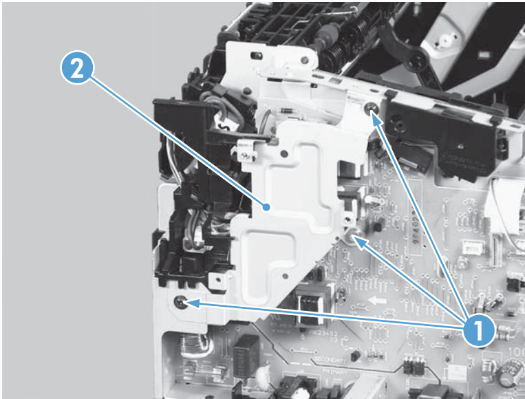
Figure 2-97 Remove the engine controller PCA (3 of 9)
