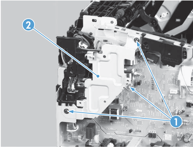
Figure 2-54 Remove the pickup assembly (4 of 10)
