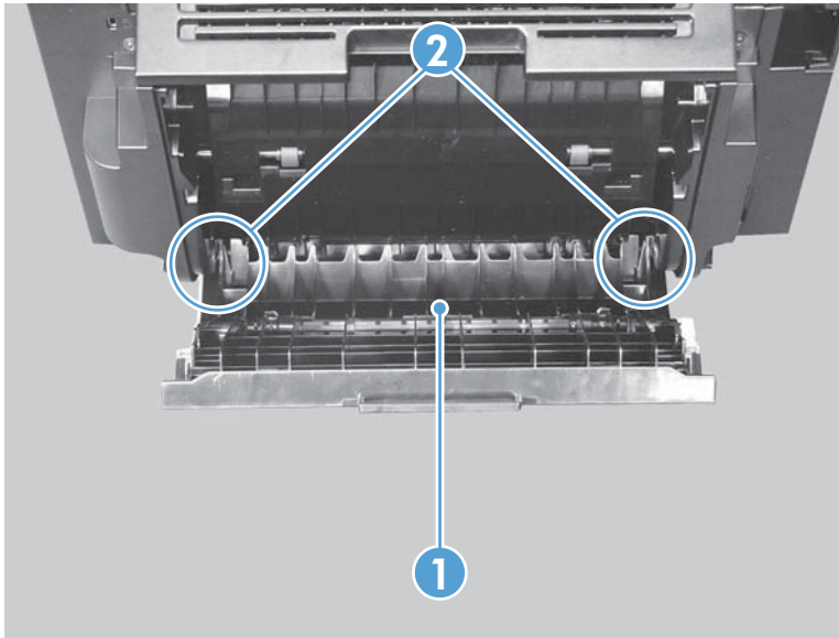
Figure 2-26 Remove the duplex door, duplex product
