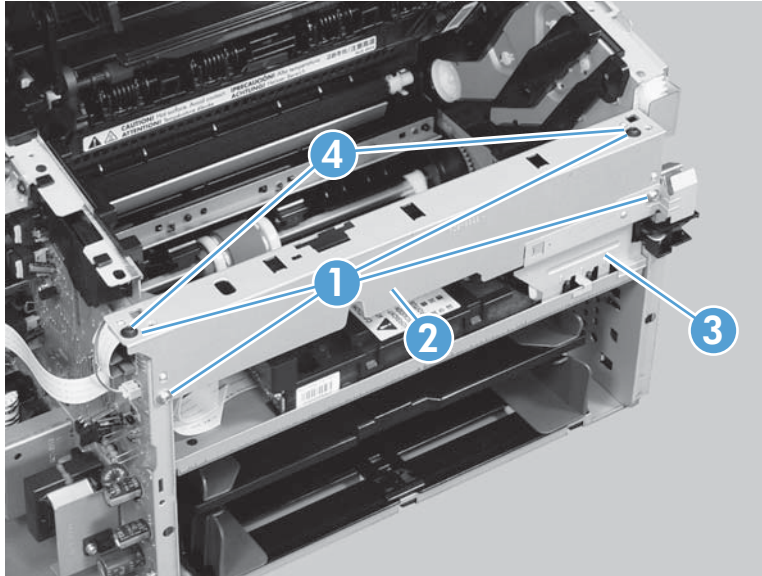
Figure 2-46 Remove the laser/scanner assembly (2 of 5)
