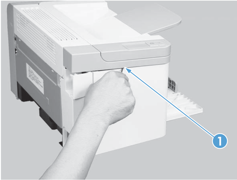
Figure 2-11 Remove the left cover, simplex product (3 of 4)
