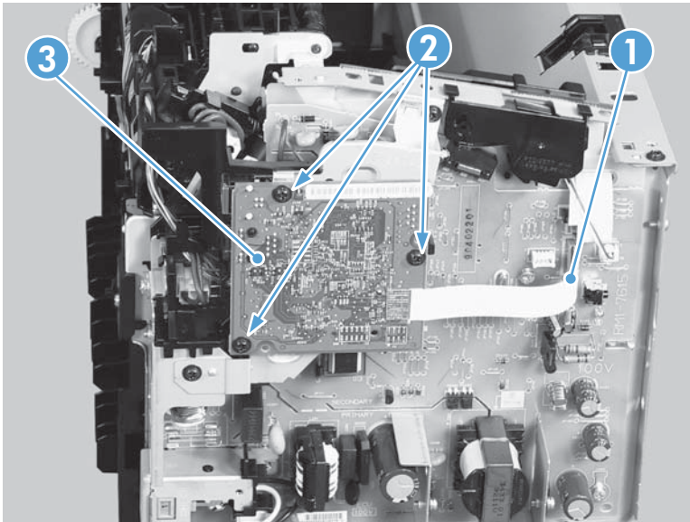
Figure 2-90 Remove the pickup solenoid (3 of 7)
