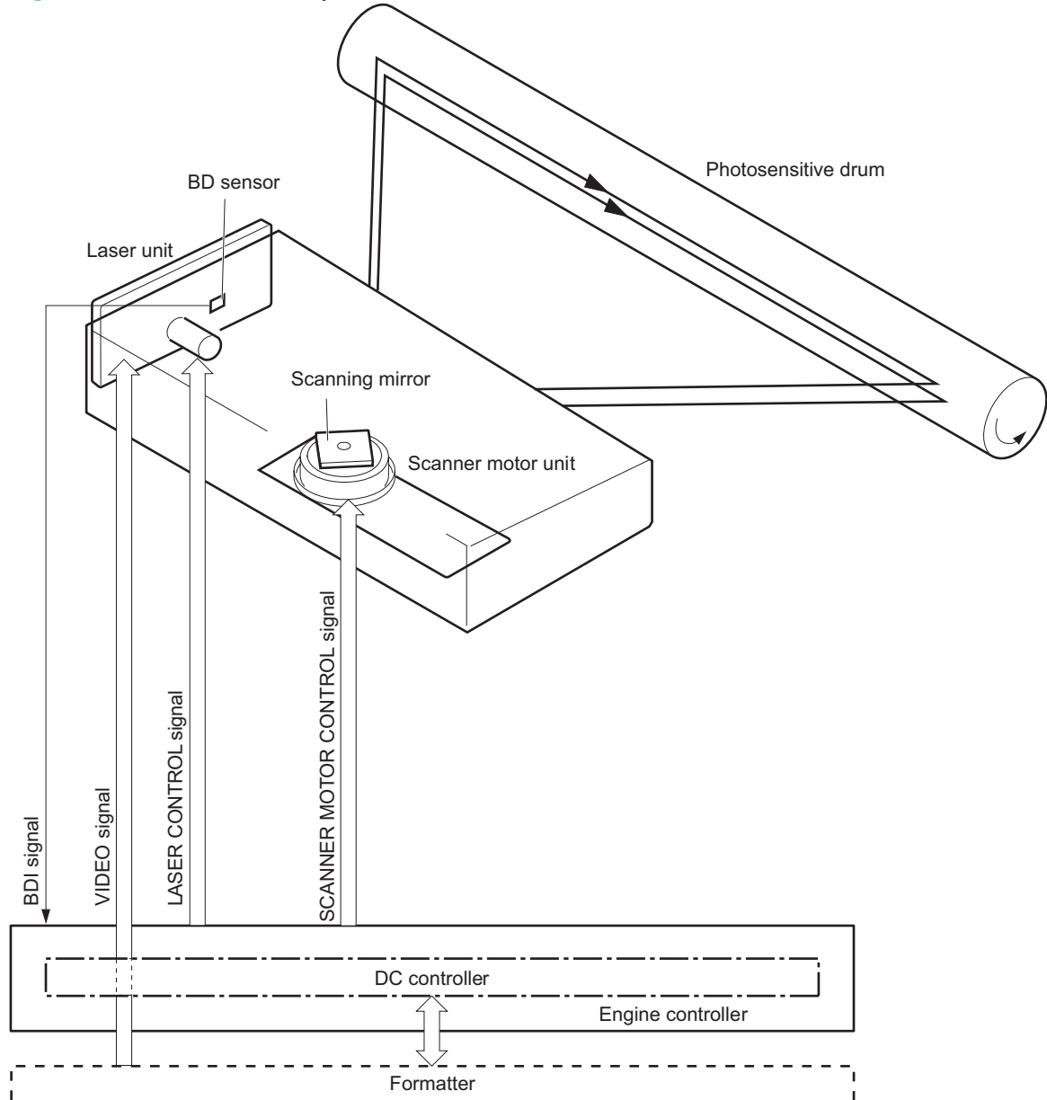
Figure 1-13 Laser/scanner system
