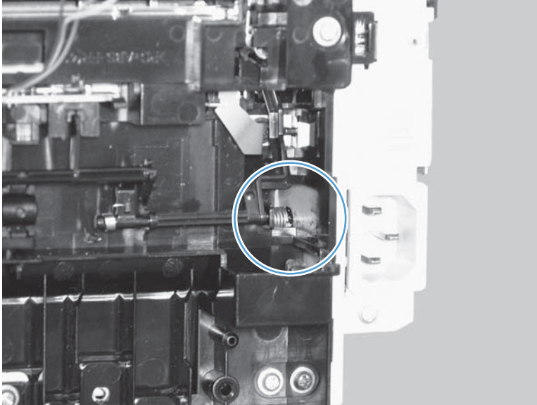
Figure 2-62 Reinstall the pickup assembly (2 of 4; incorrect ground spring position)
