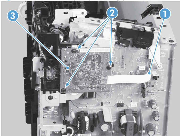
Figure 2-53 Remove the pickup assembly (3 of 10)
