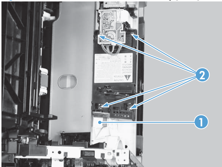
Figure 2-47 Remove the laser/scanner assembly (3 of 5)
