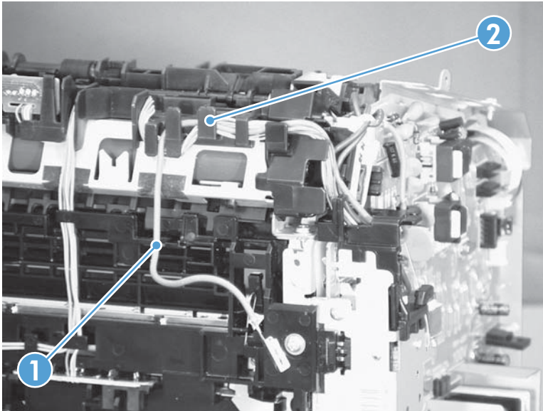
Figure 2-105 Reinstall the engine controller PCA (2 of 4)
