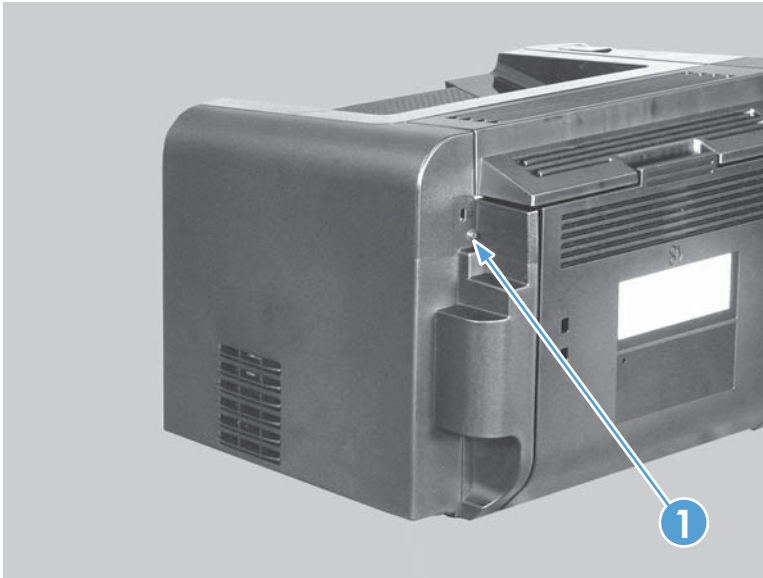
Figure 2-21 Remove the right cover, duplex product (1 of 5)
