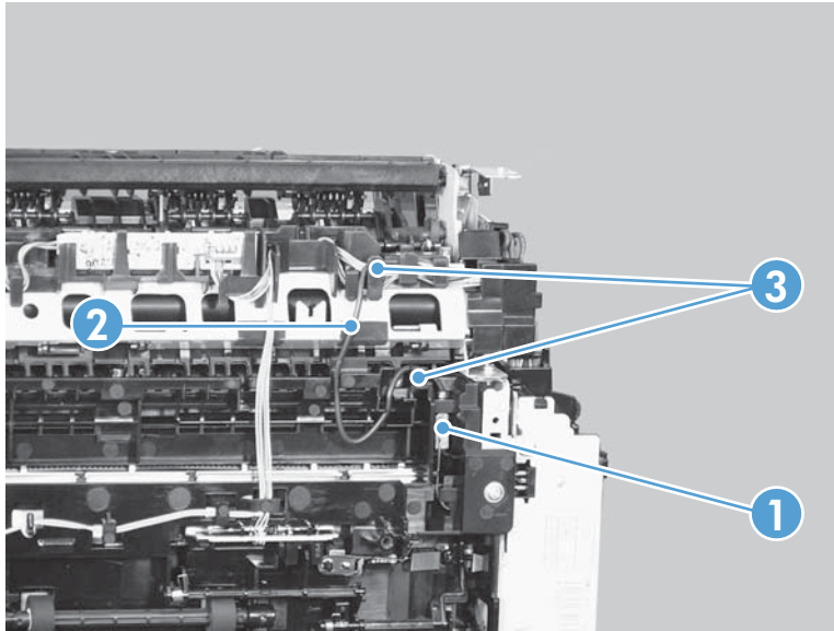
Figure 2-98 Remove the engine controller PCA (4 of 9)
