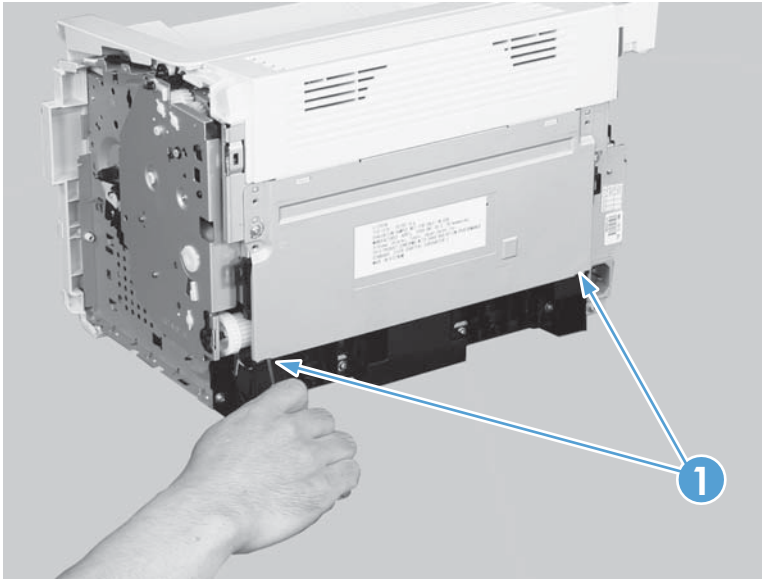
Figure 2-39 Remove the rear cover, simplex product (2 of 3)
