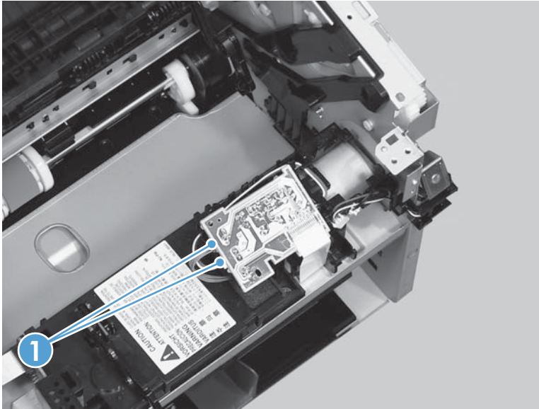
Figure 2-82 Remove the main motor (6 of 9)
