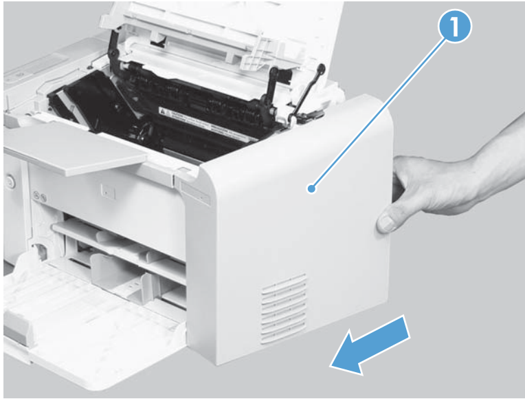
Figure 2-20 Remove the right cover, simplex product (4 of 4)
