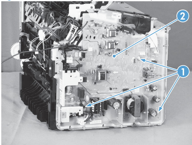
Figure 2-103 Remove the engine controller PCA (10 of 9)
