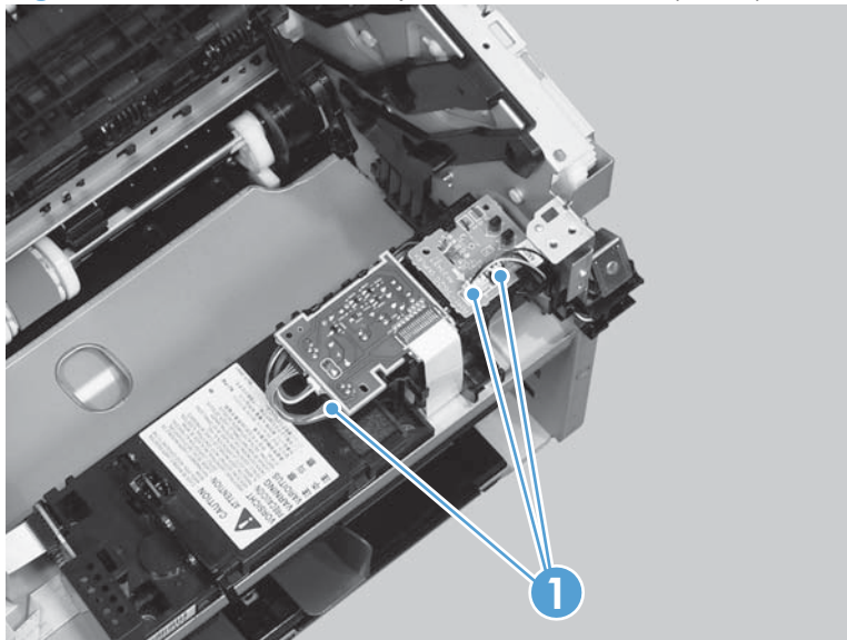
Figure 2-120 Remove the duplex-connector PCA (3 of 5)
