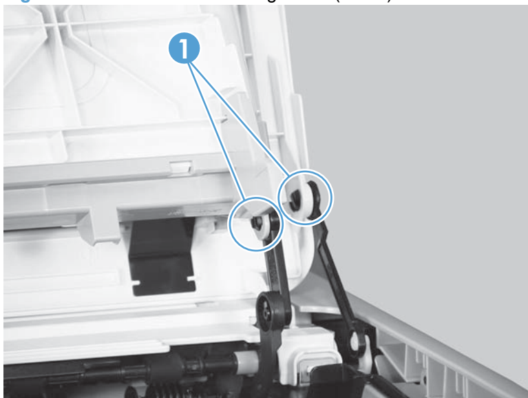
Figure 2-29 Remove the cartridge door (1 of 3)
