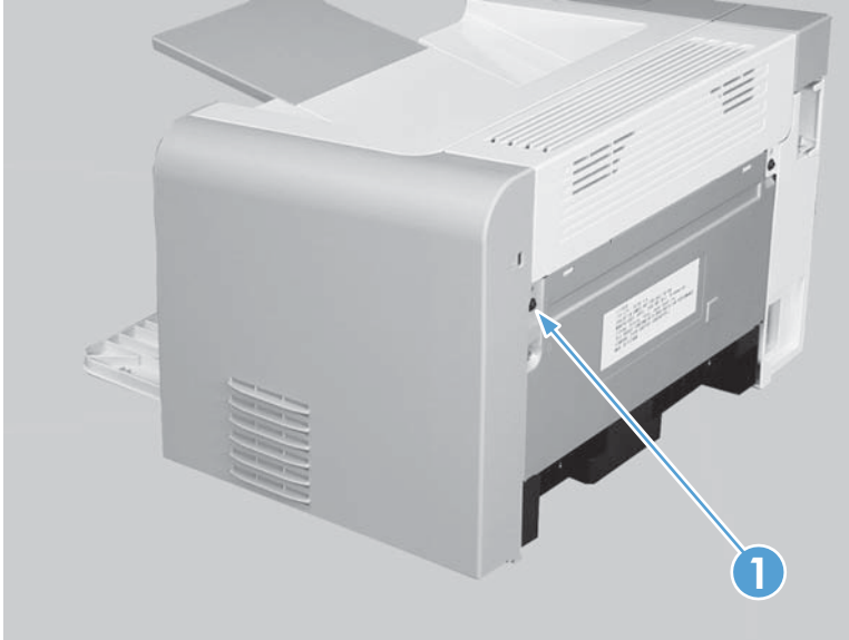
Figure 2-18 Remove the right cover, simplex product (1 of 4)
