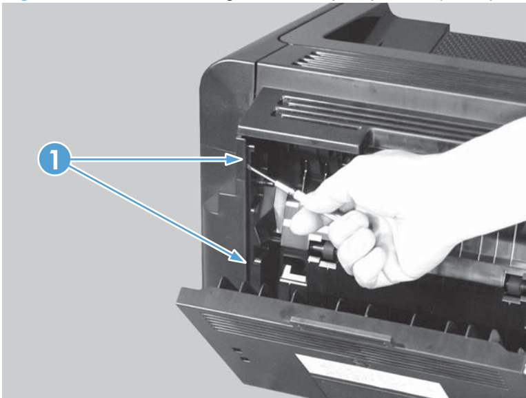
Figure 2-22 Remove the right cover, duplex product (2 of 5)
