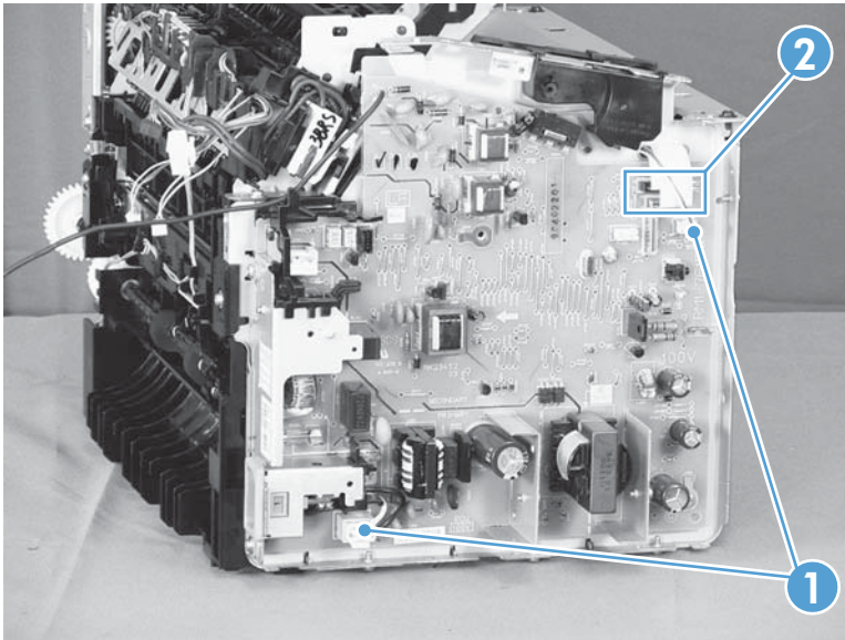
Figure 2-101 Remove the engine controller PCA (7 of 9)
