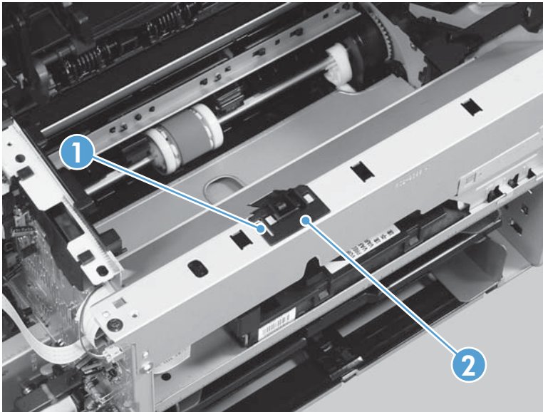
Figure 2-118 Remove the duplex-connector PCA (1 of 5)
