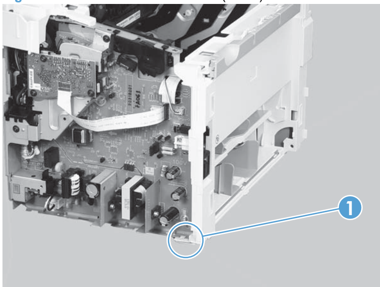
Figure 2-35 Remove the front cover (1 of 3)
