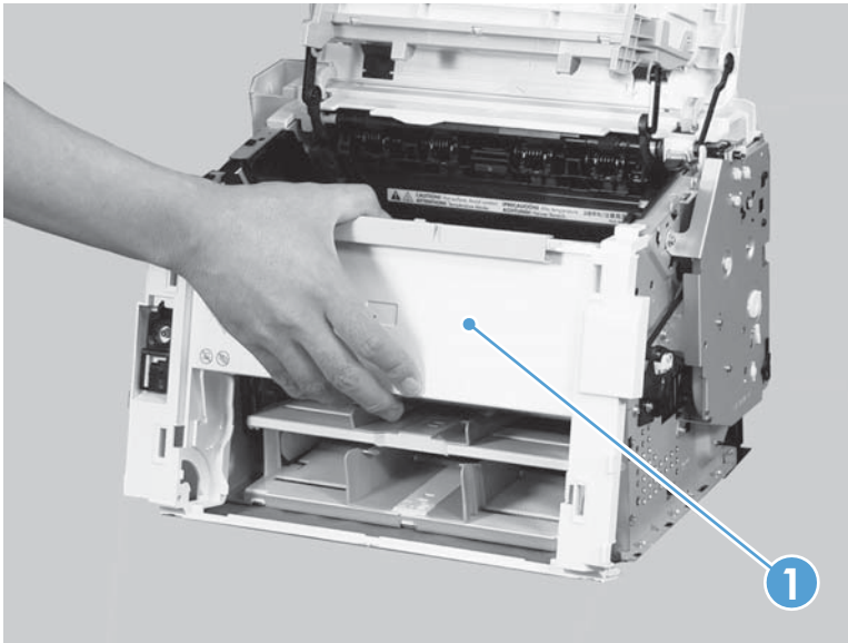
Figure 2-37 Remove the front cover (3 of 3)
