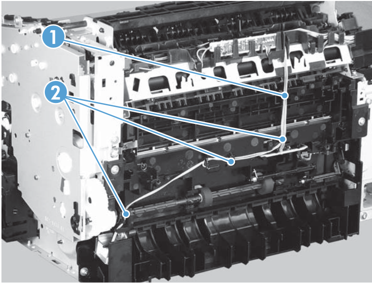
Figure 2-93 Remove the pickup solenoid (6 of 7)
