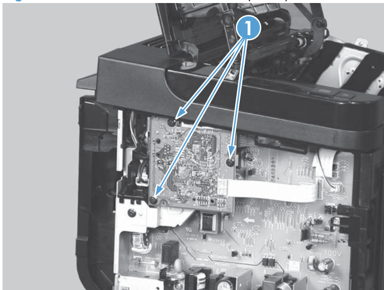
Figure 2-44 Remove the formatter PCA (2 of 2)
