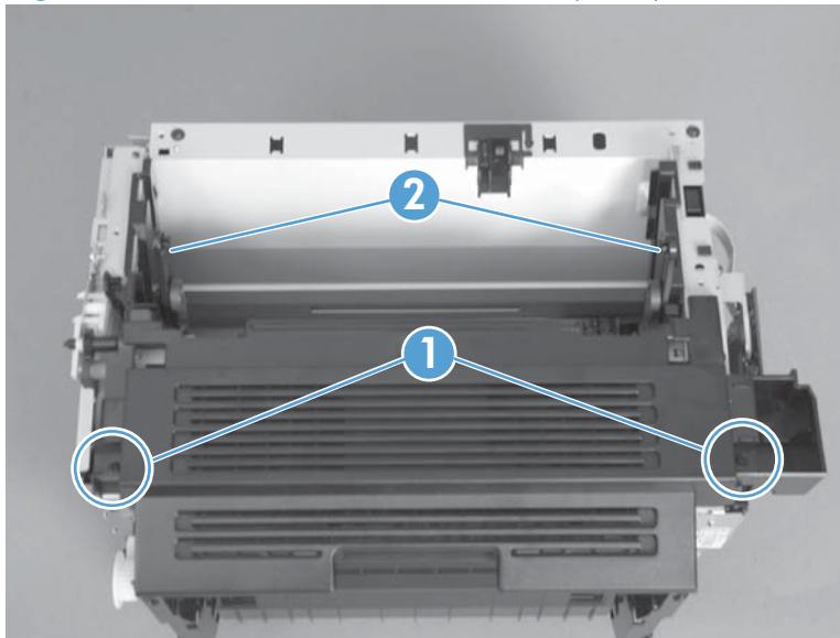
Figure 2-41 Remove the face-down cover (1 of 2)
