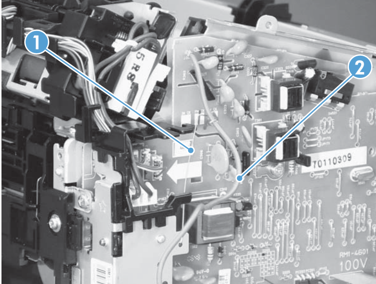
Figure 2-104 Reinstall the engine controller PCA (1 of 4)
