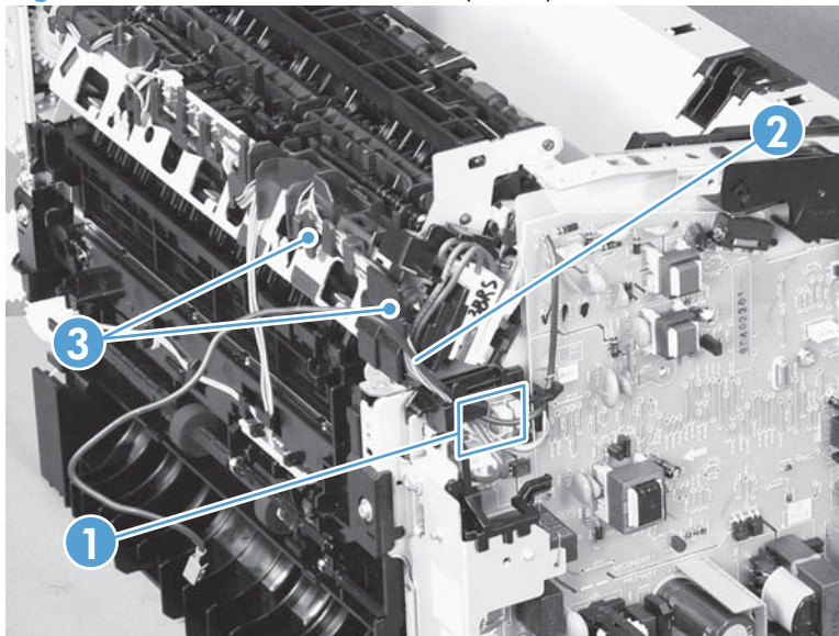
Figure 2-92 Remove the solenoid (5 of 7)
