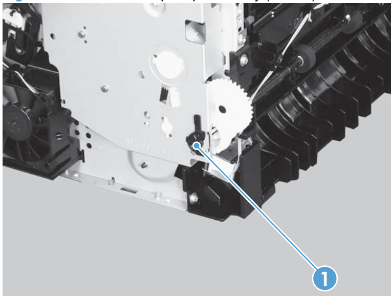
Figure 2-57 Remove the pickup assembly (7 of 10)
