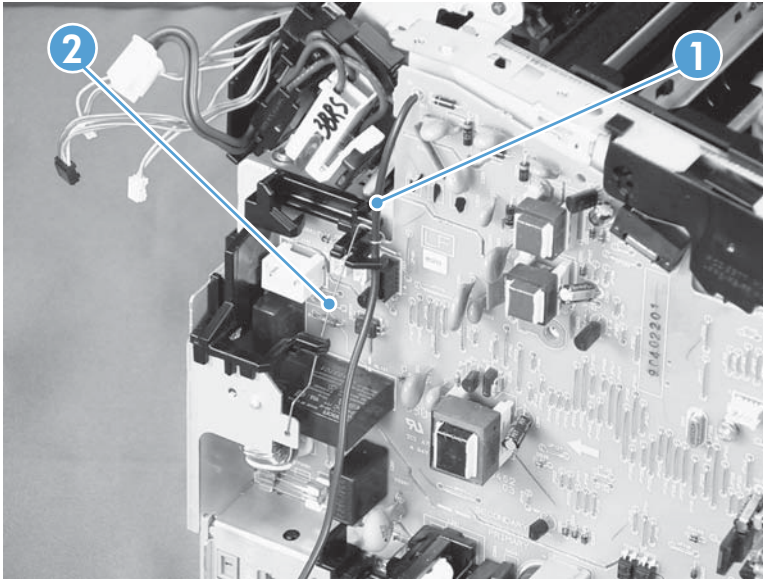
Figure 2-100 Remove the engine controller PCA (6 of 9)
