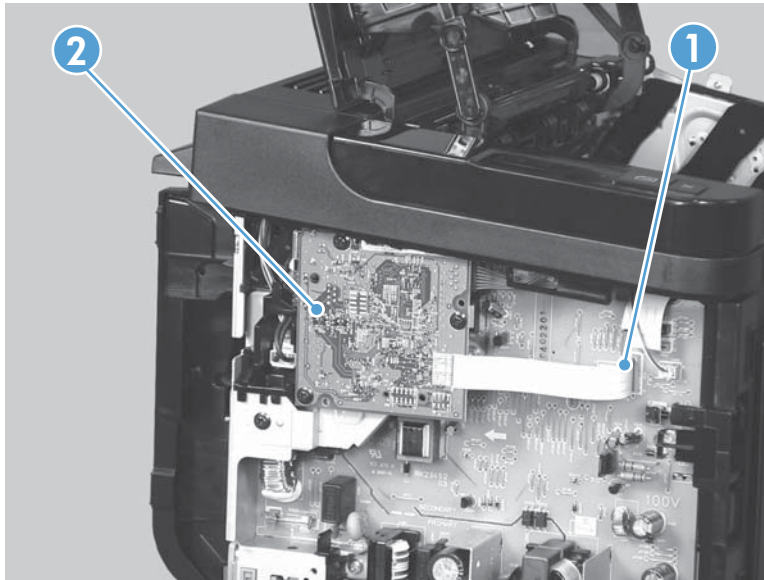
Figure 2-43 Remove the formatter PCA (1 of 2)
