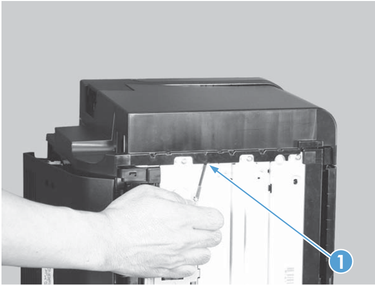
Figure 2-15 Remove the left cover, duplex product (3 of 5)
