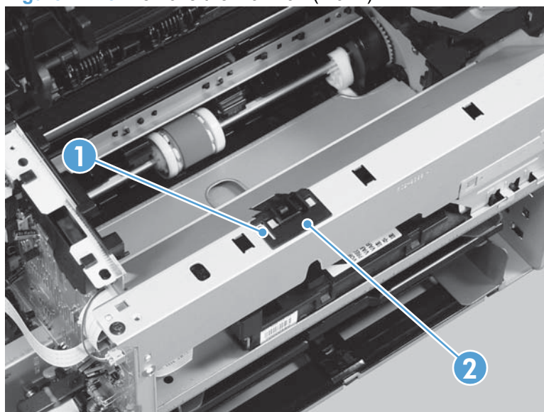
Figure 2-113 Remove the main fan (1 of 4)
