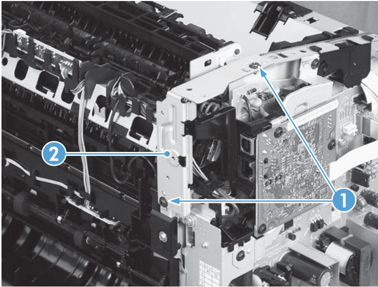
Figure 2-89 Remove the pickup solenoid (2 of 7)
