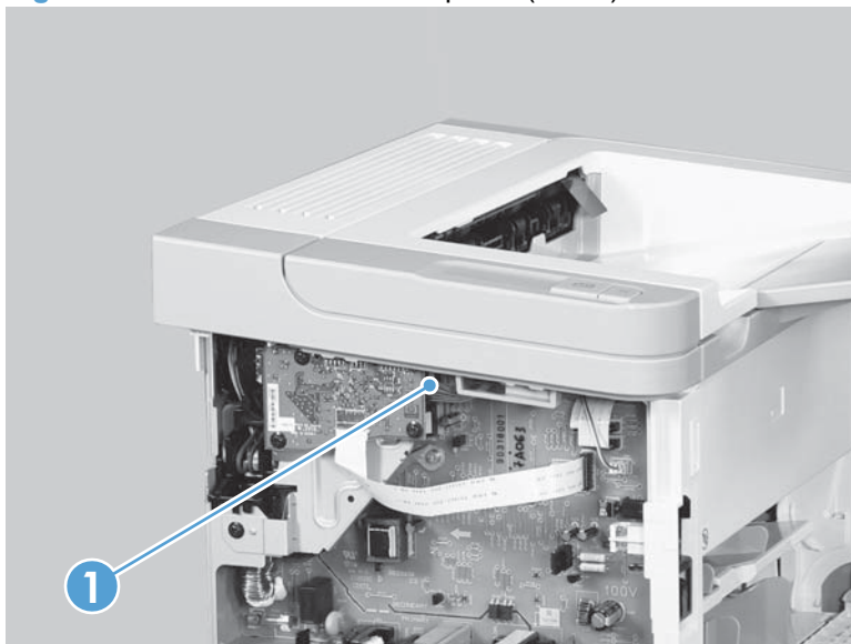
Figure 2-33 Remove the control panel (2 of 3)
