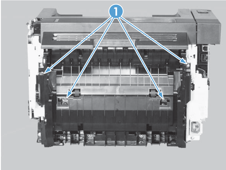
Figure 2-27 Remove the duplex frame (1 of 2)
