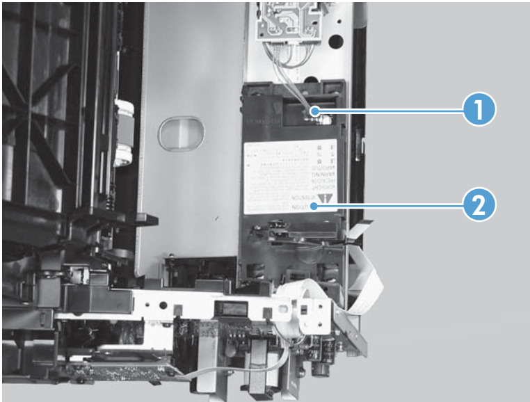
Figure 2-49 Remove the laser/scanner assembly (5 of 5)
