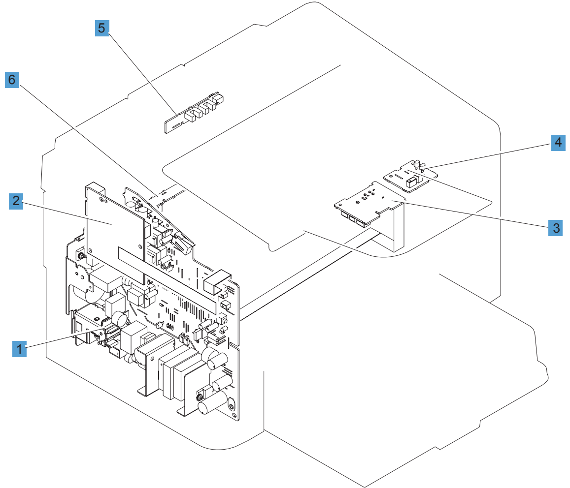
Figure 4-7 PCAs
