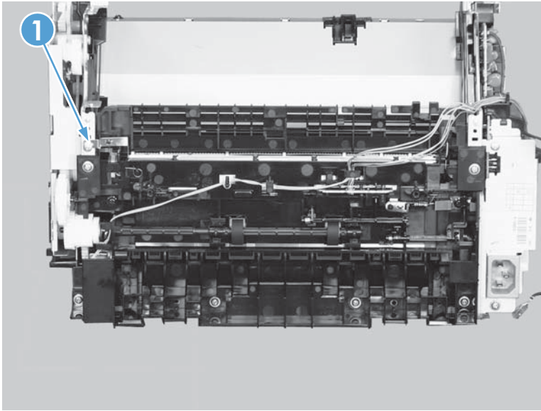
Figure 2-58 Remove the pickup assembly (8 of 10)
