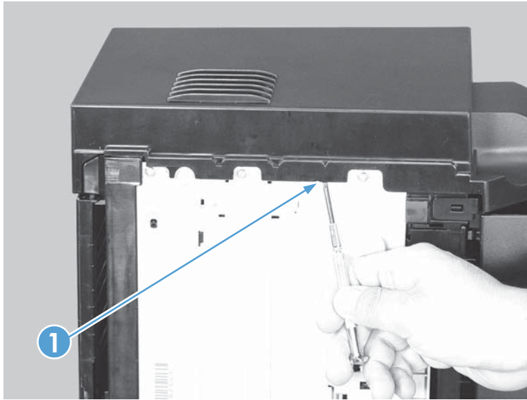
Figure 2-23 Remove the right cover, duplex product (3 of 5)
