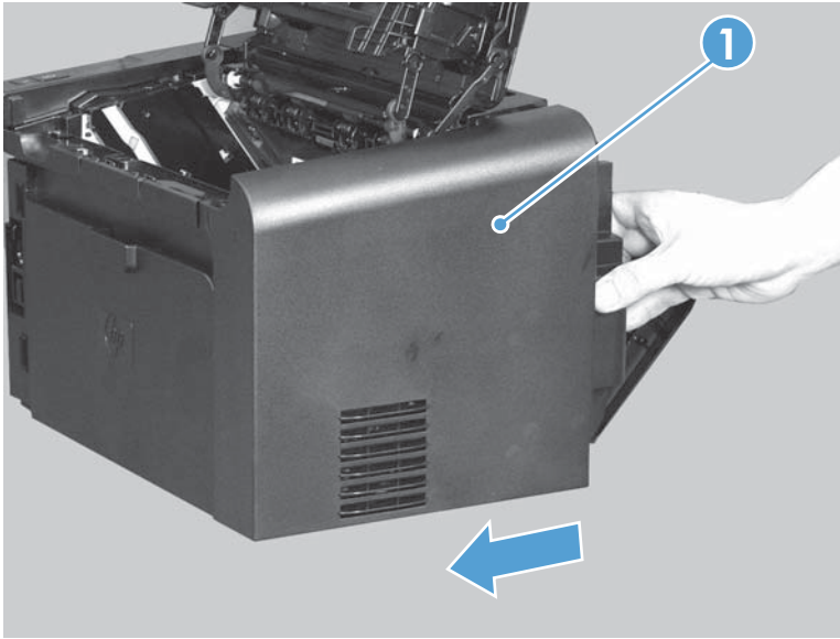
Figure 2-25 Remove the right cover, duplex product (5 of 5)
