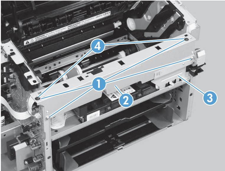
Figure 2-78 Remove the main motor (2 of 9)
