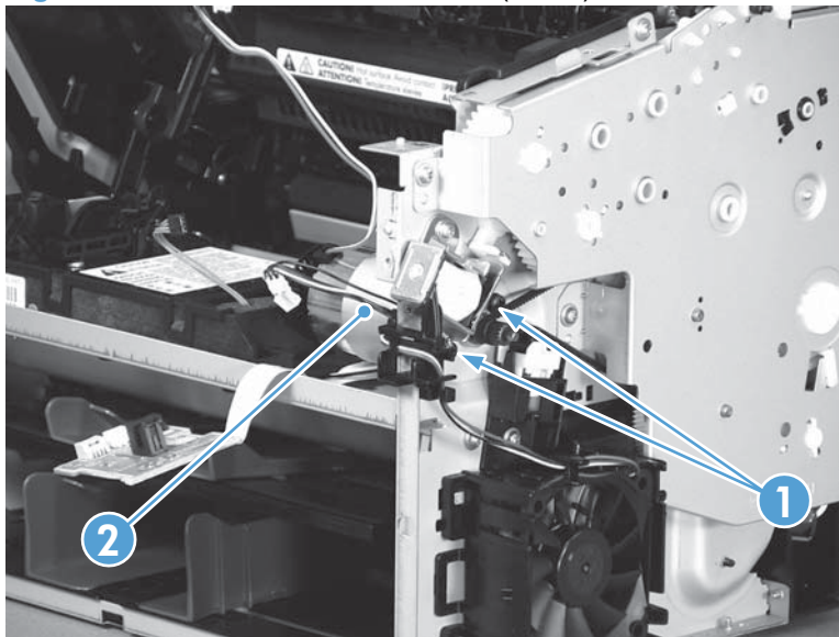
Figure 2-85 Remove the main motor (9 of 9)
