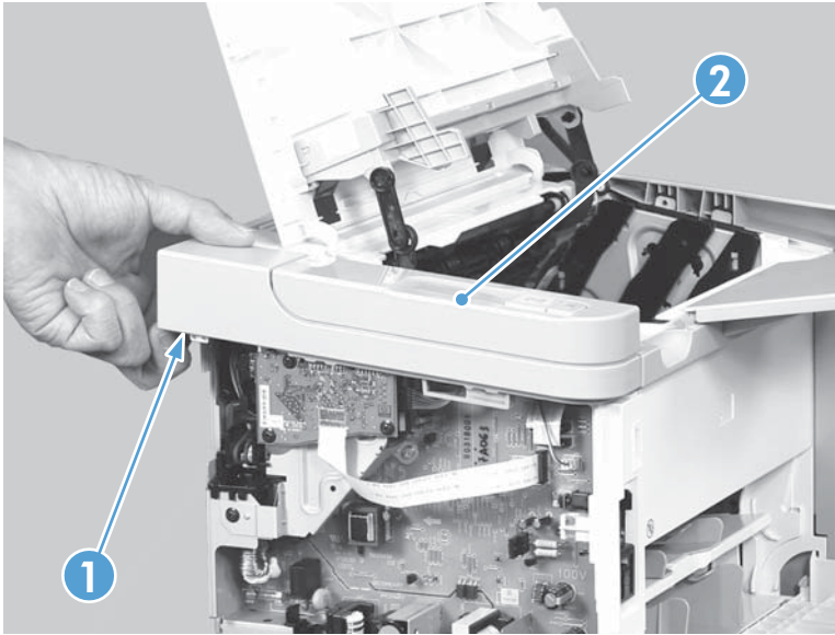
Figure 2-34 Remove the control panel (3 of 3)
