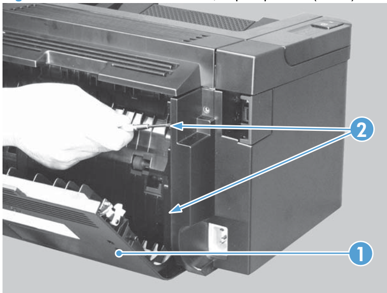
Figure 2-14 Remove the left cover, duplex product (2 of 5)
