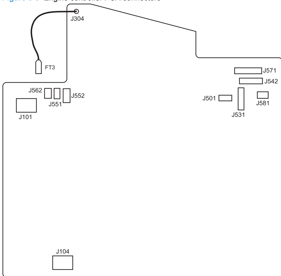
Figure 3-3 Engine controller PCA connectors
