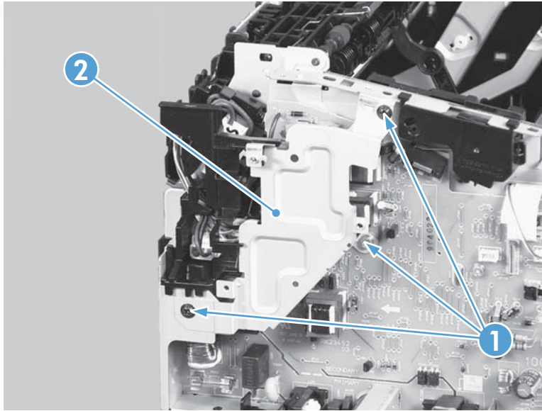
Figure 2-91 Remove the pickup solenoid (4 of 7)
