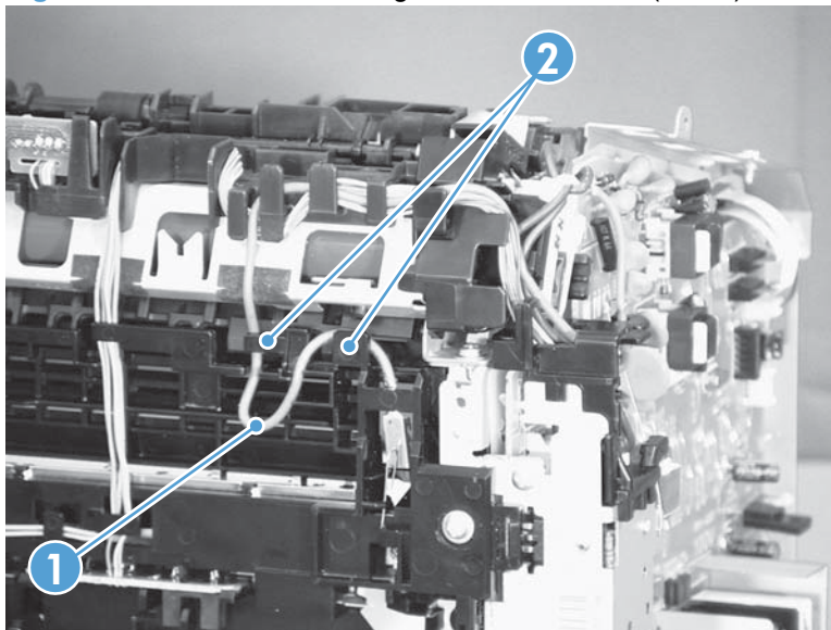
Figure 2-107 Reinstall the engine controller PCA (4 of 4)
