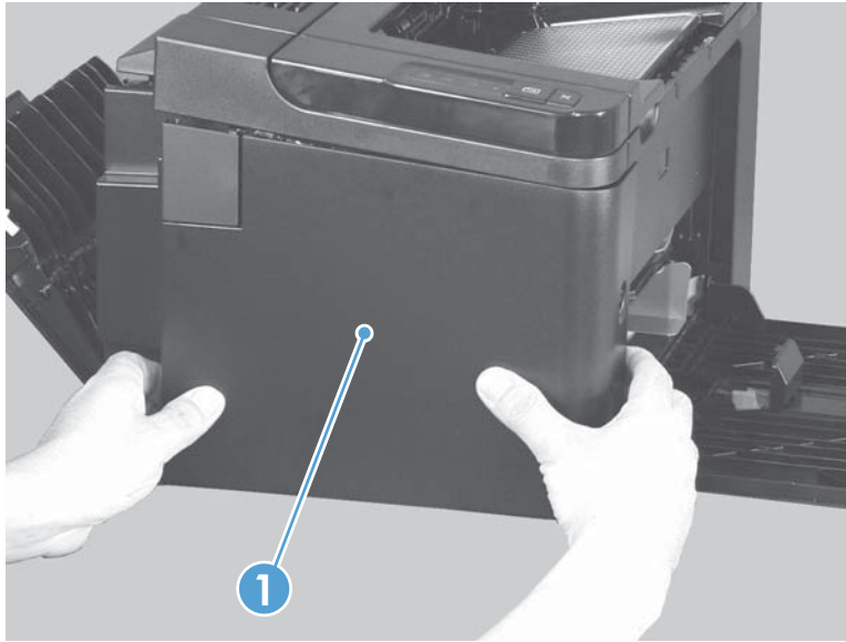
Figure 2-17 Remove the left cover, duplex product (5 of 5)
