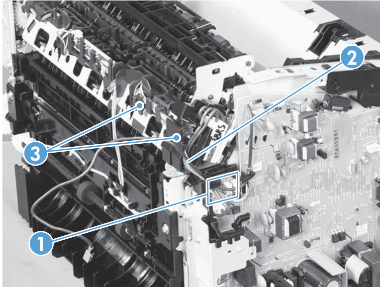
Figure 2-56 Remove the pickup assembly (6 of 10)
