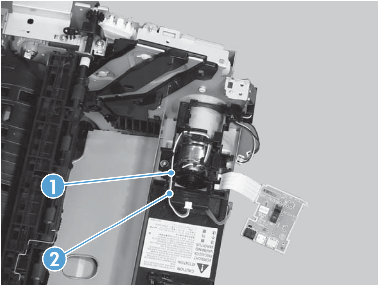
Figure 2-83 Remove the main motor (7 of 9)
