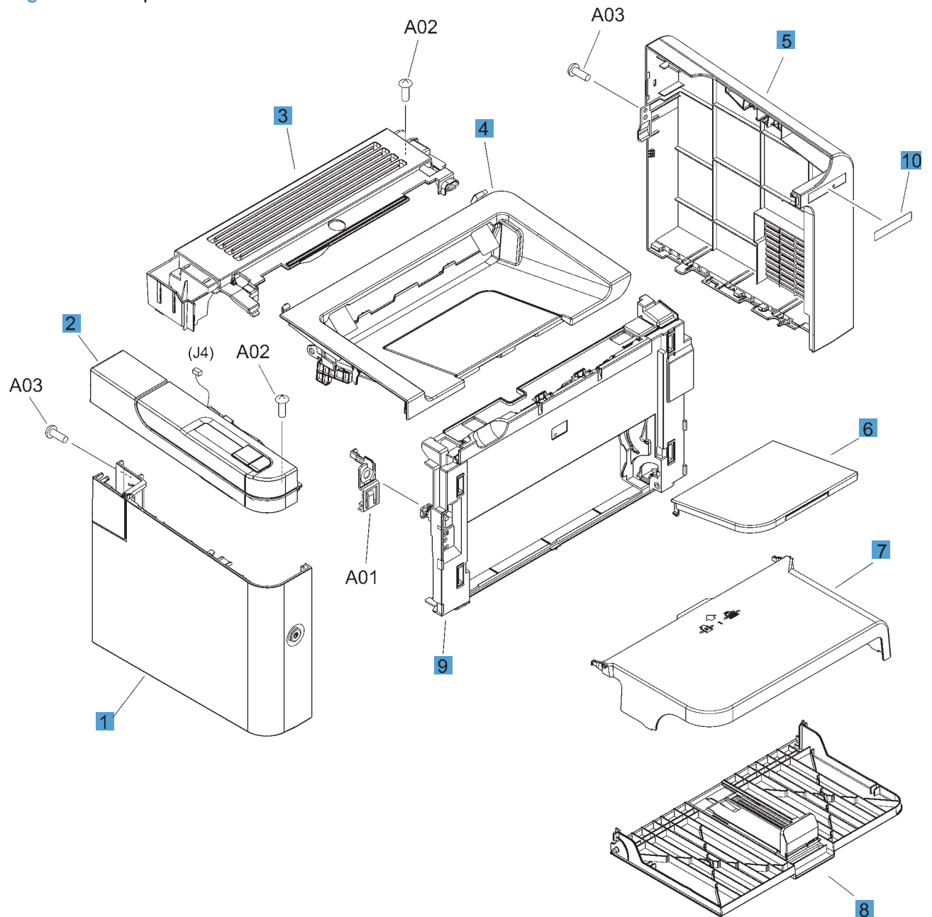
Figure 4-2 Simplex model
