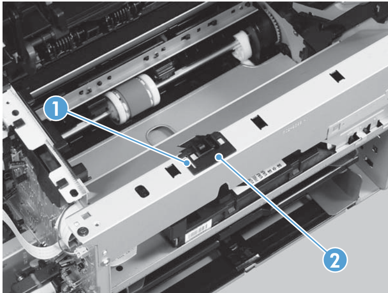
Figure 2-45 Remove the laser/scanner assembly (1 of 5)
