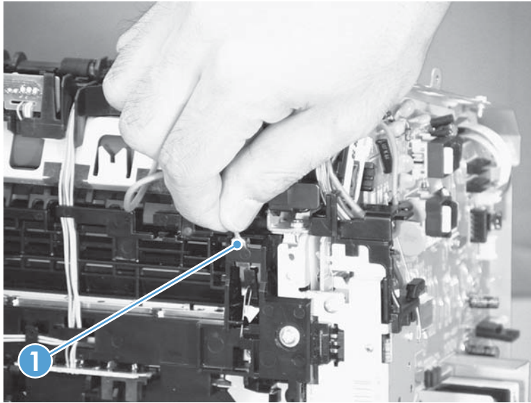
Figure 2-106 Reinstall the engine controller PCA (3 of 4)
