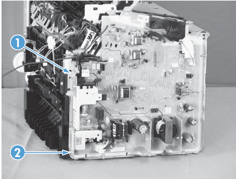
Figure 2-102 Remove the engine controller PCA (8 of 9)
