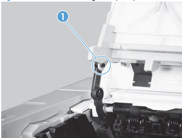
Figure 2-30 Remove the cartridge door (2 of 3)
