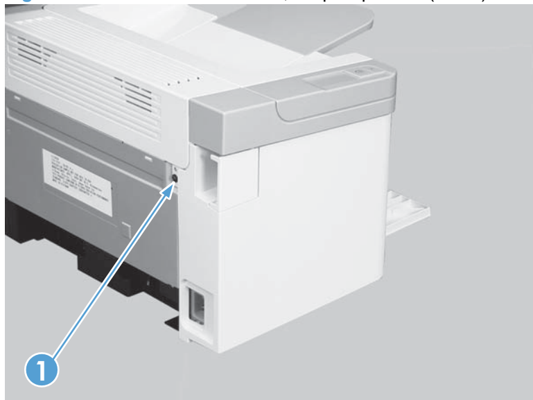
Figure 2-9 Remove the left cover, simplex product (1 of 4)
