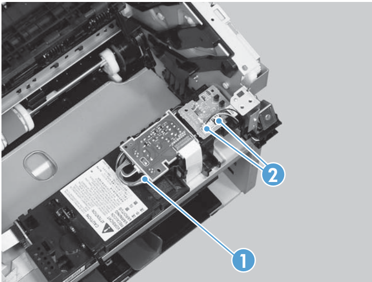
Figure 2-79 Remove the main motor (3 of 9)
