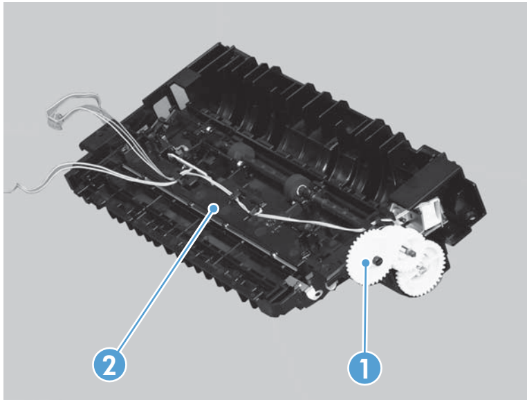
Figure 2-60 Remove the pickup assembly (10 of 10)
