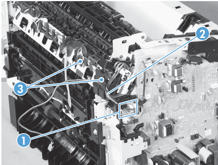
Figure 2-99 Remove the engine controller PCA (5 of 9)
