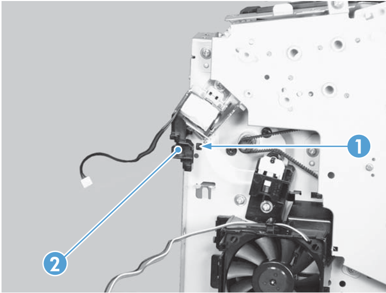
Figure 2-111 Remove the duplex-reverse solenoid (4 of 5)
