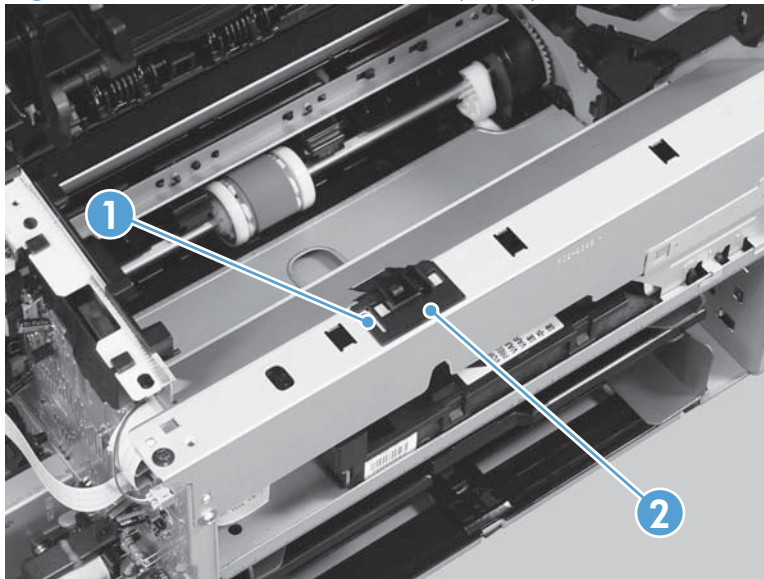
Figure 2-77 Remove the main motor (1 of 9)
