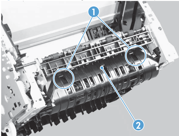
Figure 2-95 Remove the engine controller PCA (1 of 9)
