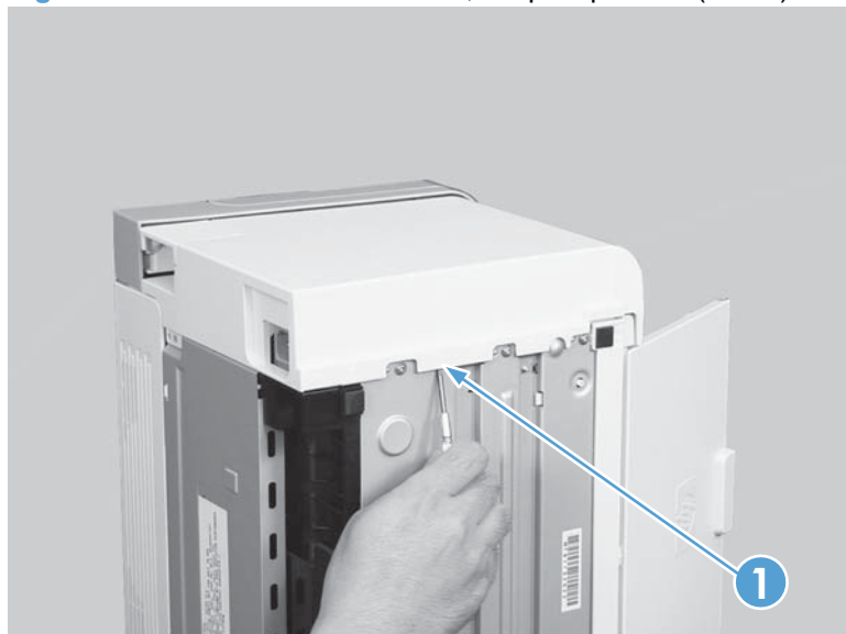
Figure 2-10 Remove the left cover, simplex product (2 of 4)
