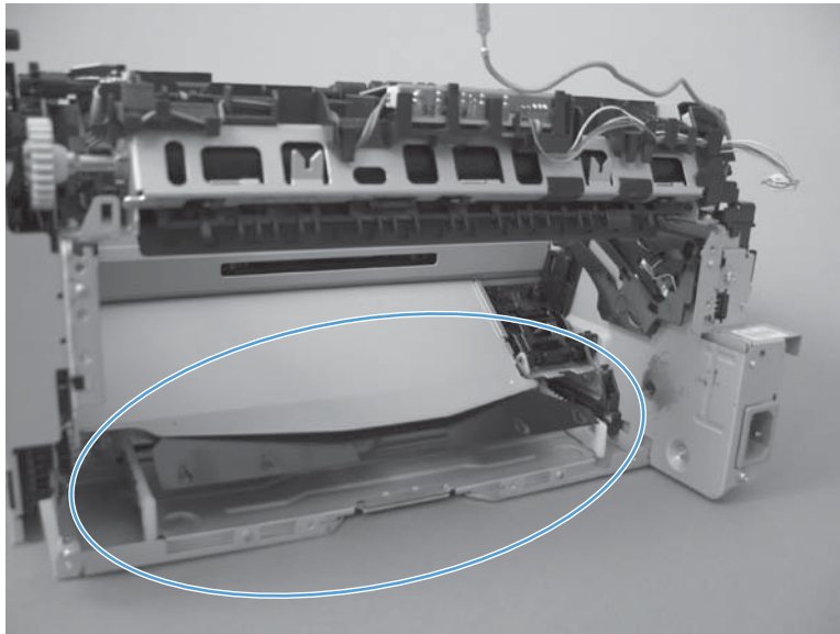
Figure 2-64 Reinstall the pickup assembly (4 of 4; lift plate in lowered position)
