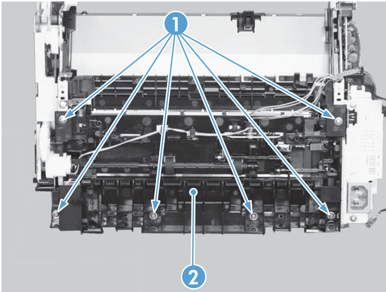
Figure 2-59 Remove the pickup assembly (9 of 10)
