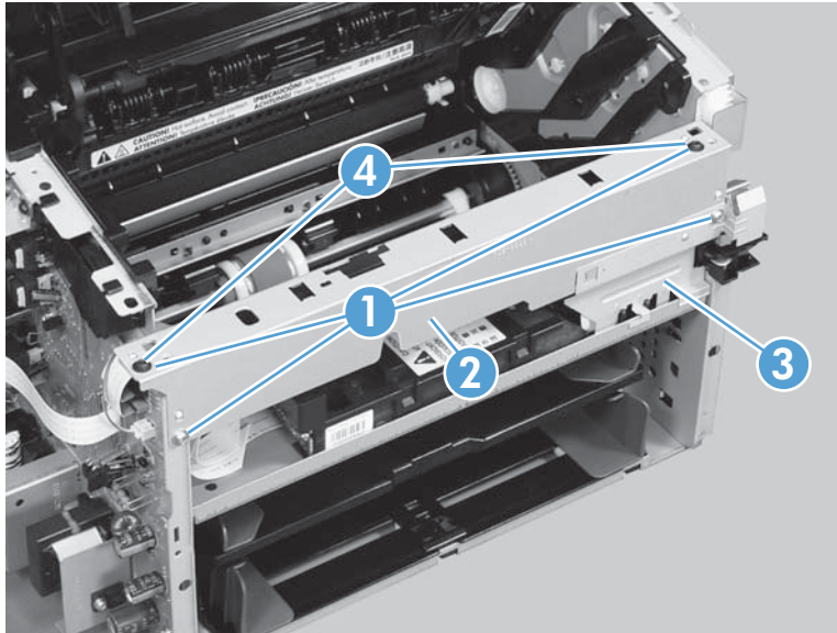
Figure 2-119 Remove the duplex-connector PCA (2 of 5)
