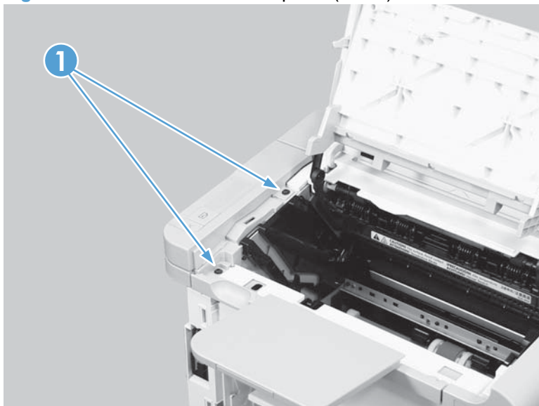
Figure 2-32 Remove the control panel (1 of 3)
