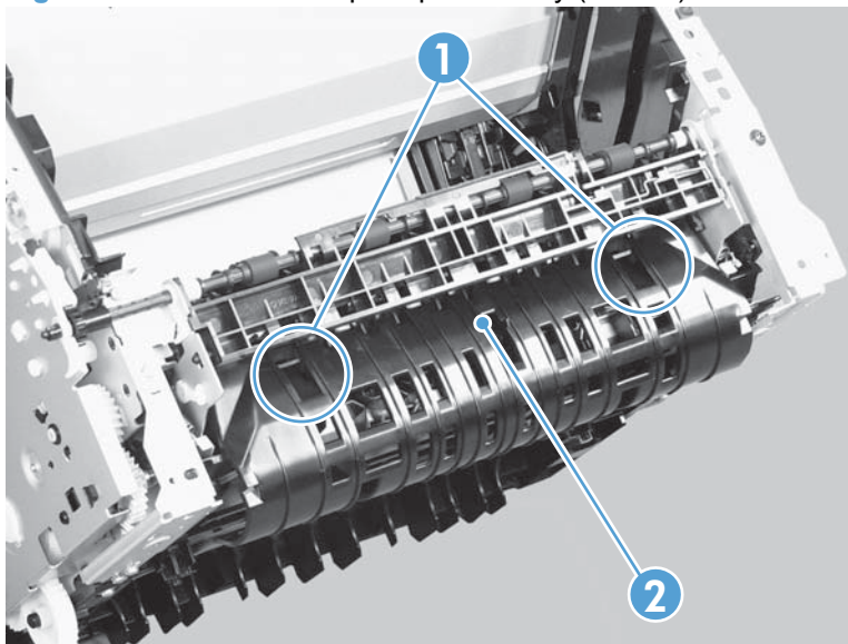
Figure 2-51 Remove the pickup assembly (1 of 10)
