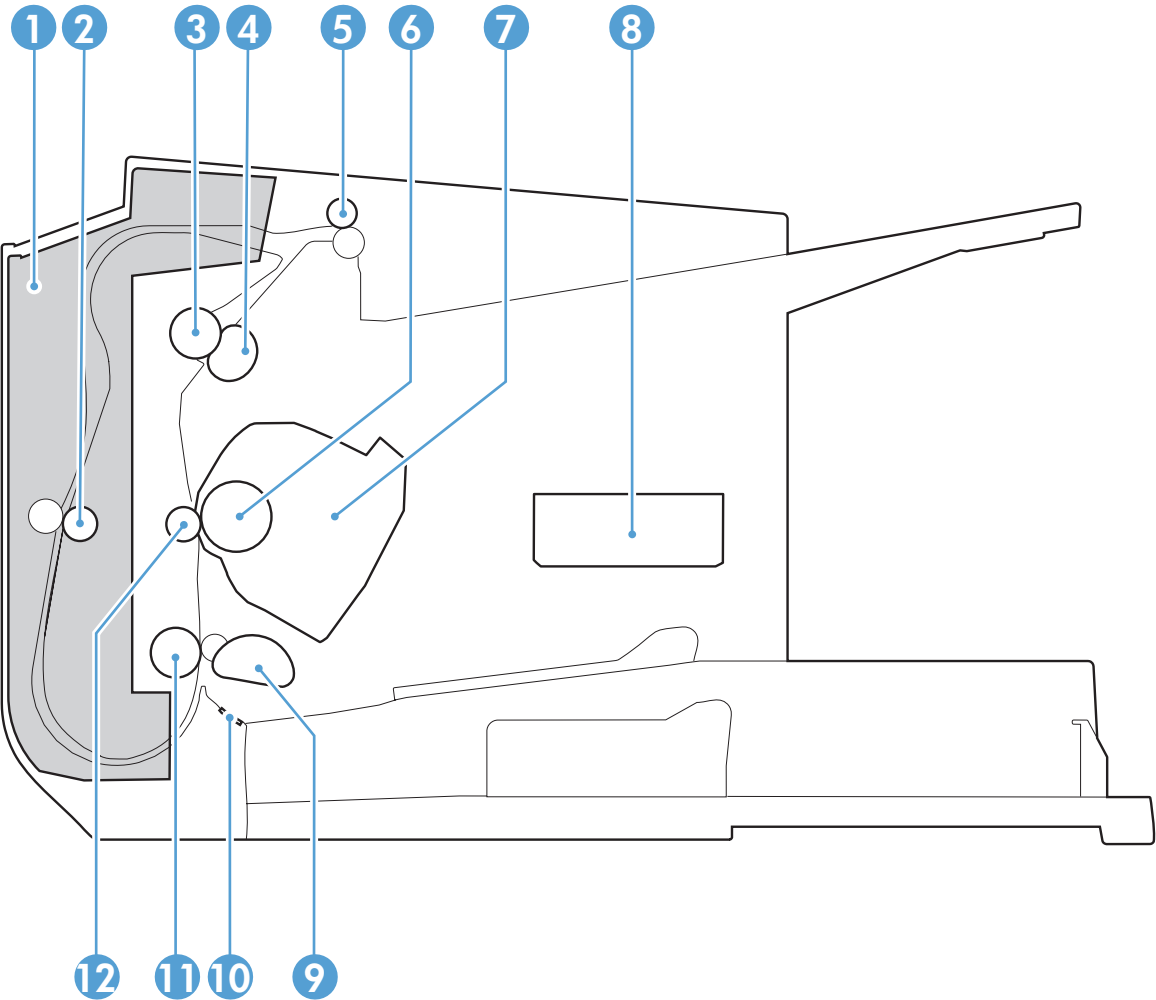
Figure 3-5 Cross section view
