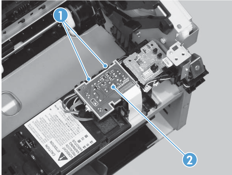
Figure 2-80 Remove the main motor (4 of 9)
