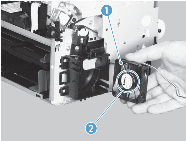
Figure 2-117 Reinstall the main fan
