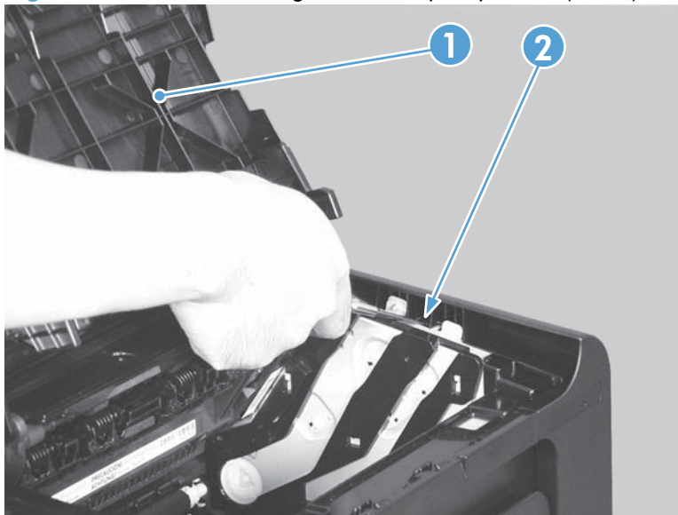
Figure 2-24 Remove the right cover, duplex product (4 of 5)
