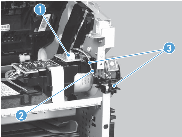
Figure 2-115 Remove the main fan (3 of 4)
