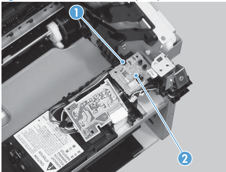
Figure 2-81 Remove the main motor (5 of 9)
