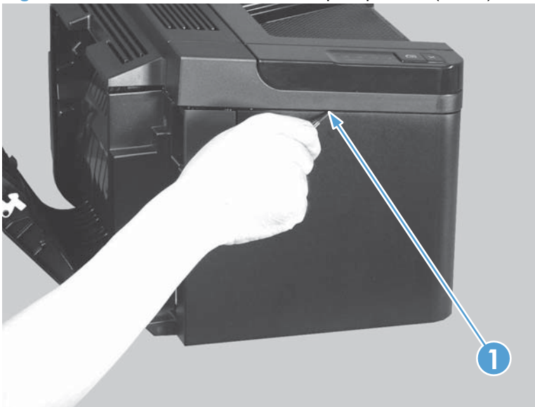
Figure 2-16 Remove the left cover, duplex product (4 of 5)
