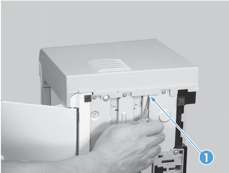
Figure 2-19 Remove the right cover, simplex product (2 of 4)
