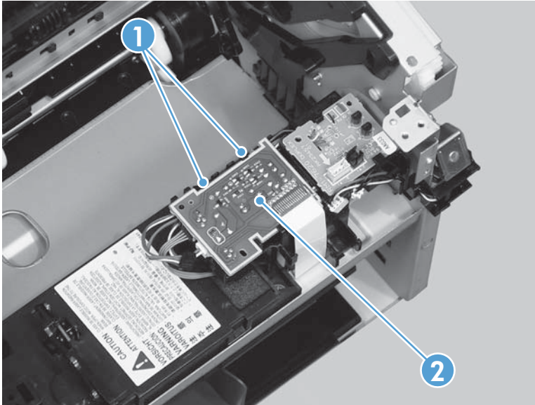
Figure 2-121 Remove the duplex-connector PCA (4 of 5)
