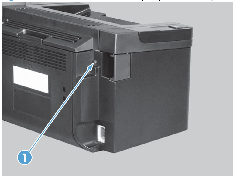
Figure 2-13 Remove the left cover, duplex product (1 of 5)
