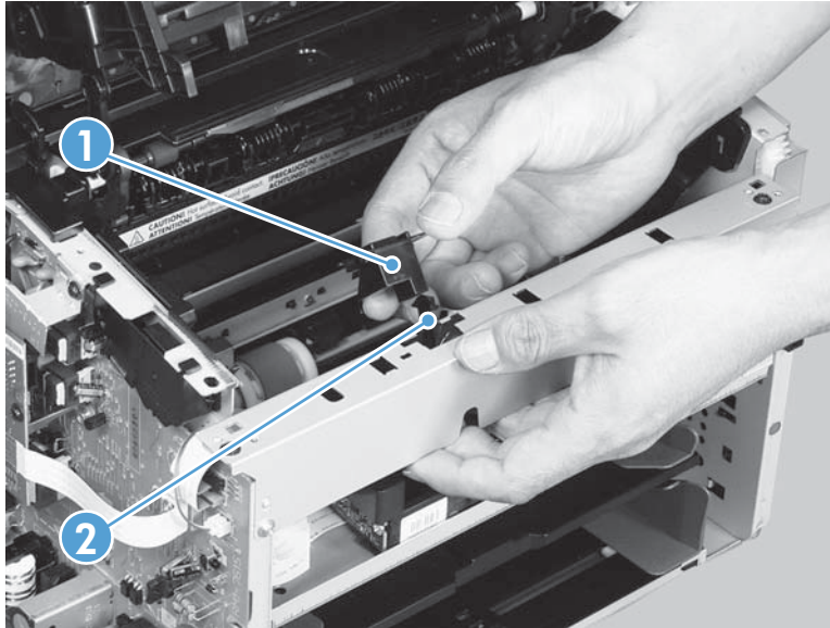
Figure 2-50 Reinstall the laser/scanner assembly
