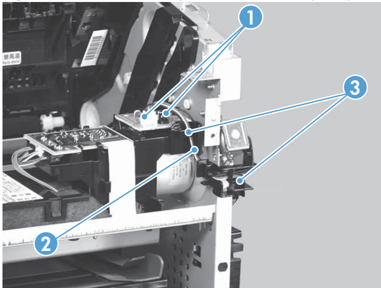
Figure 2-110 Remove the duplex-reverse solenoid (3 of 5)
