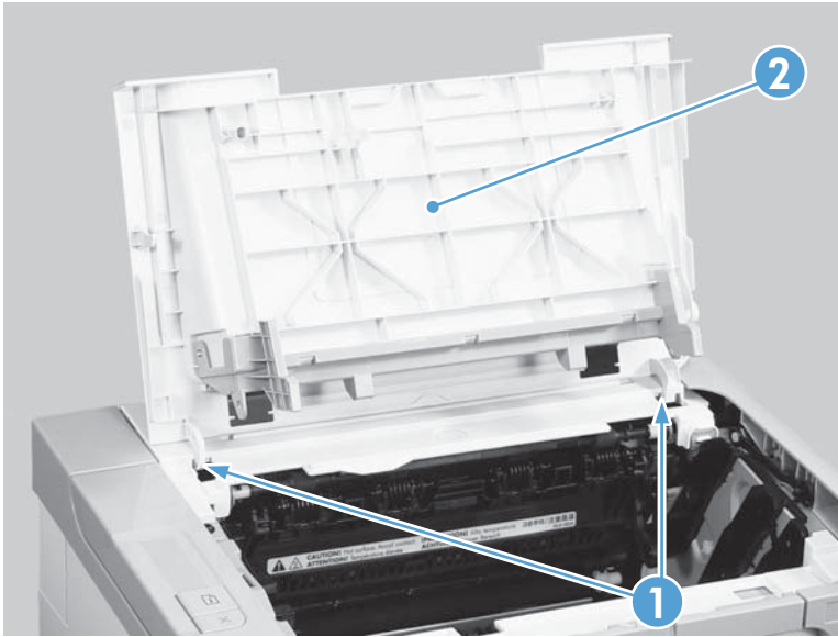
Figure 2-31 Remove the cartridge door (3 of 3)
