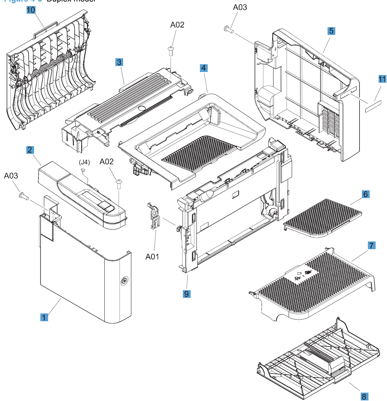
Figure 4-3 Duplex model
