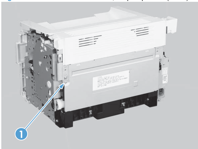
Figure 2-38 Remove the rear cover, simplex product (1 of 3)
