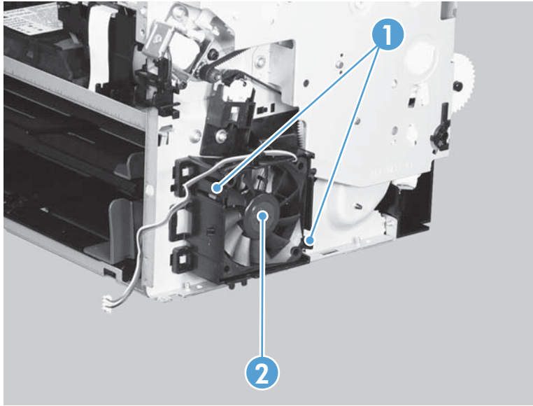
Figure 2-116 Remove the main fan (4 of 4)
