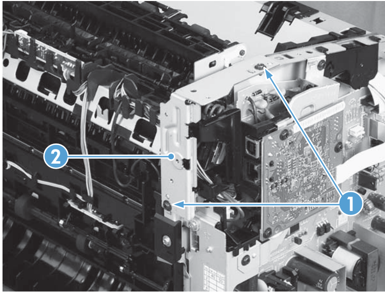
Figure 2-52 Remove the pickup assembly (2 of 10)
