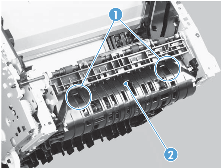
Figure 2-88 Remove the pickup solenoid (1 of 7)
