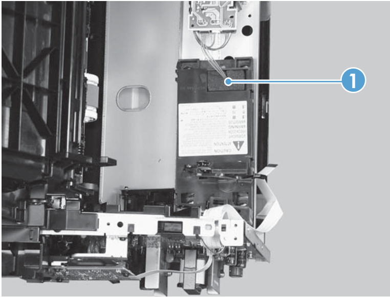
Figure 2-48 Remove the laser/scanner assembly (4 of 5)
