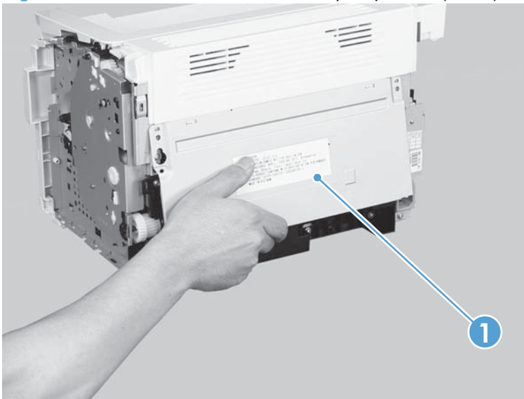
Figure 2-40 Remove the rear cover, simplex product (2 of 3)
