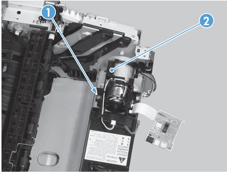
Figure 2-84 Remove the main motor (8 of 9)
