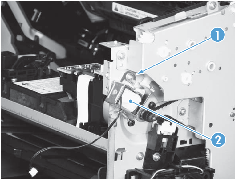
Figure 2-112 Remove the duplex-reverse solenoid (5 of 5)
