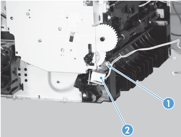
Figure 2-94 Remove the pickup solenoid (7 of 7)
