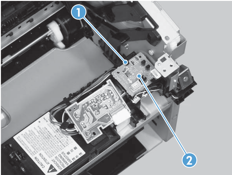
Figure 2-122 Remove the duplex-connector PCA (5 of 5)
