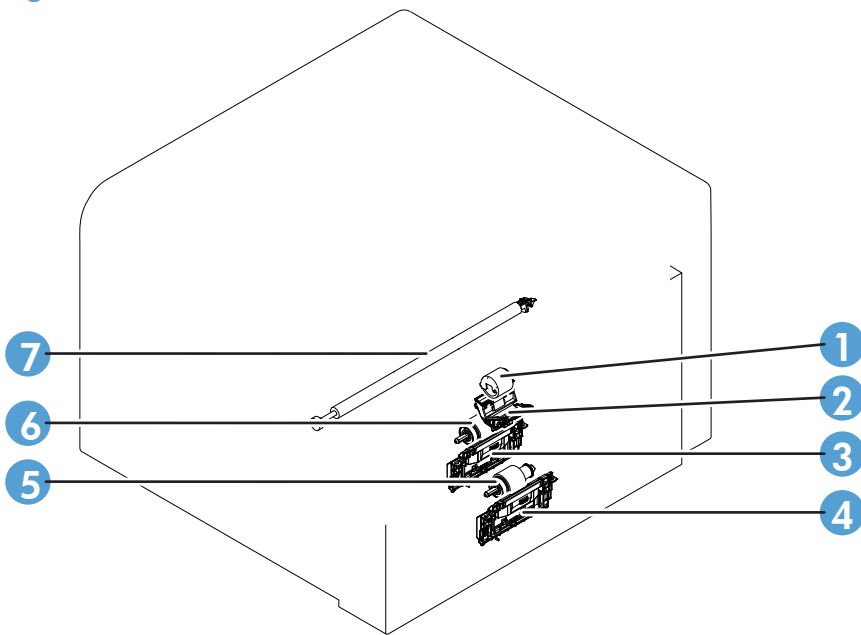
Figure 2-60 Roller locations
