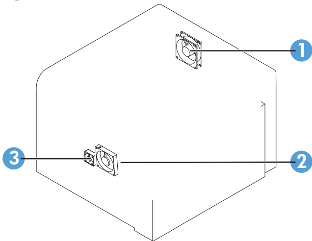
Figure 2-59 Fan locations
