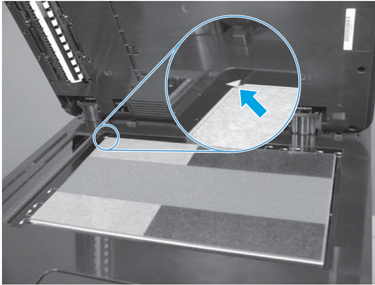
Figure 1-86 Install a replacement document feeder white backing (5 of 9)
