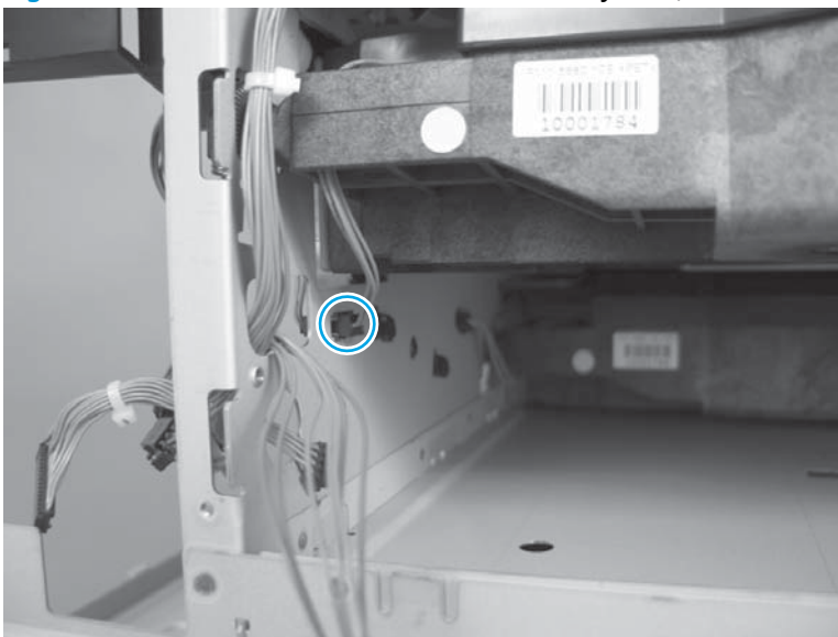
Figure 1-353 Remove the laser/scanner assembly (Y/M; 2 of 5)
