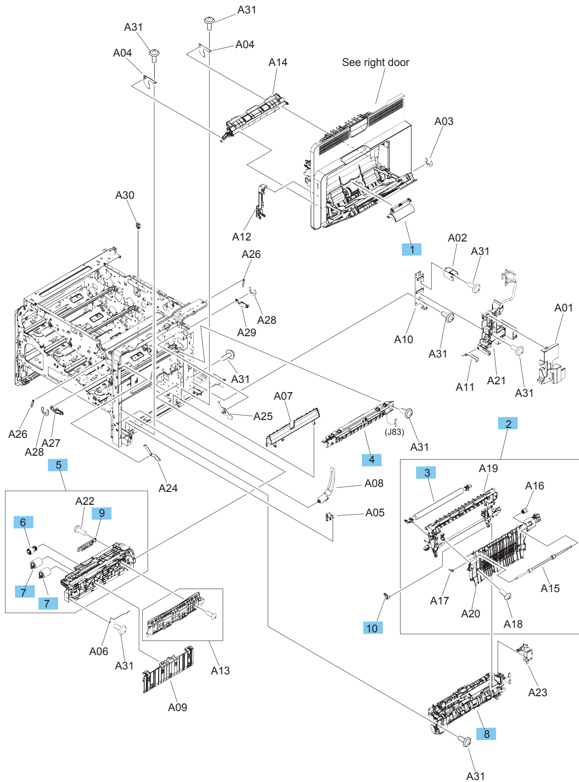
Figure 2-14 Internal assemblies (4 of 6)
