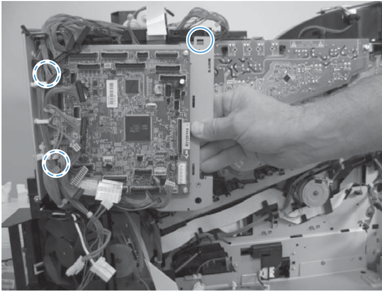
Figure 1-316 Remove the DC controller PCA and tray (3 of 3)
