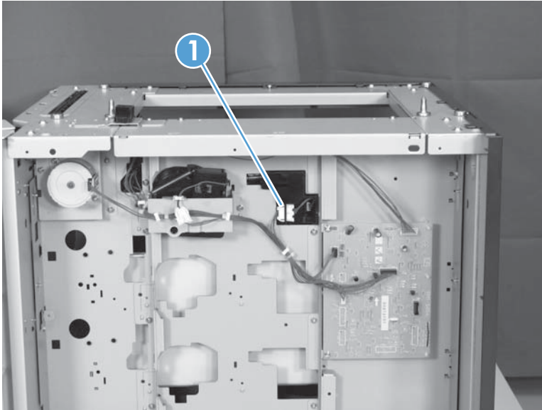
Figure 1-434 Remove the lifter base assembly (1x500-sheet paper feeder with cabinet; 1 of 2)
