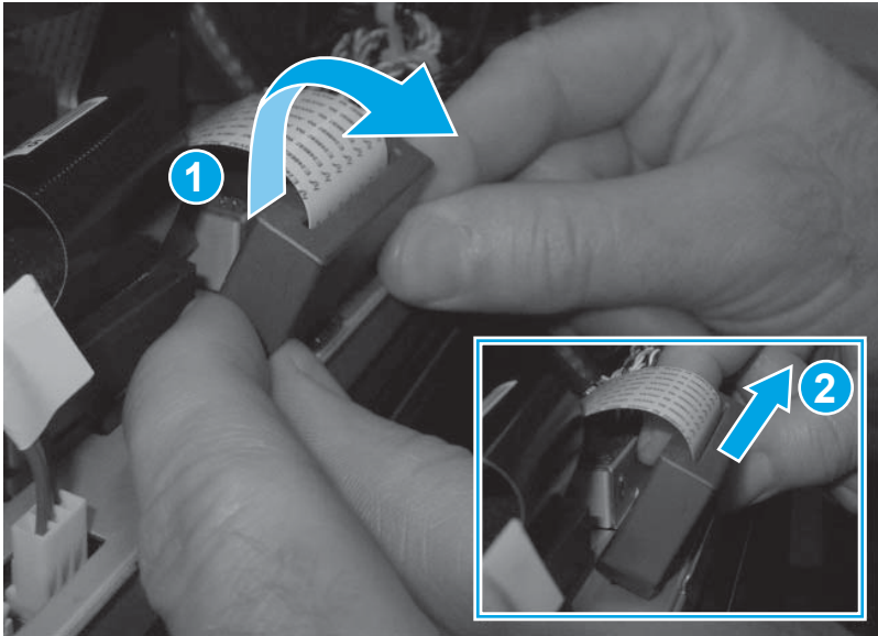
Figure 1-169 Transfer the SCB to the replacement scanner assembly (4 of 6)
