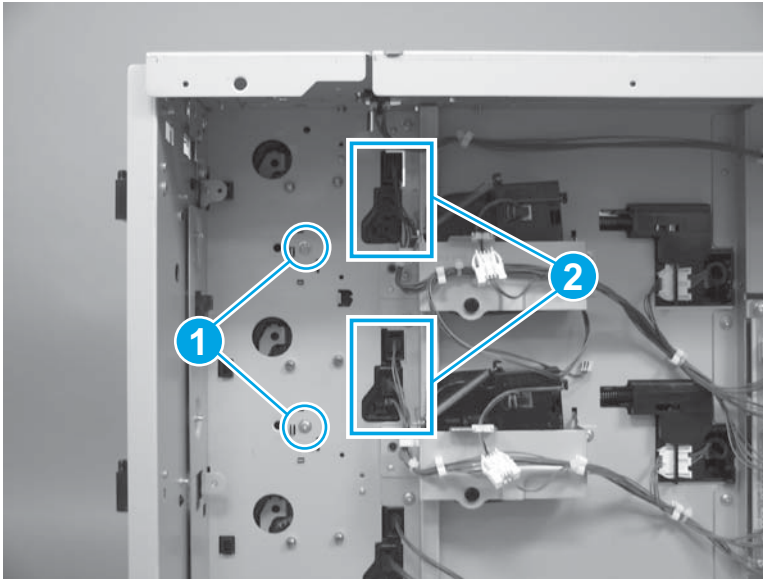
Figure 1-458 Remove the Tray 3-4 pickup assemblies (2,500-sheet paper feeder HCl; 3 of 4)
