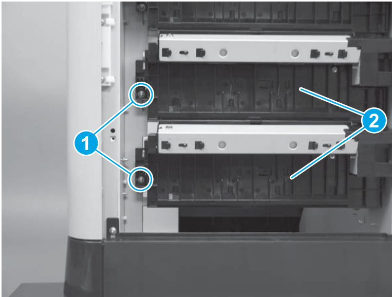
Figure 1-459 Remove the Tray 3-4 pickup assemblies (2,500-sheet paper feeder HCl; 4 of 4)
