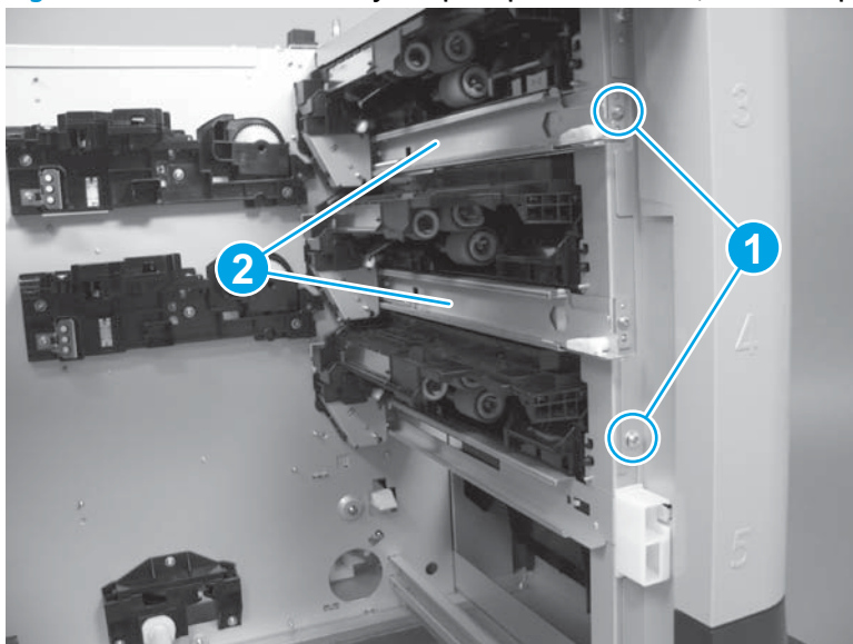
Figure 1-456 Remove the Tray 3-4 pickup assemblies (2,500-sheet paper feeder HCI; 1 of 4)
