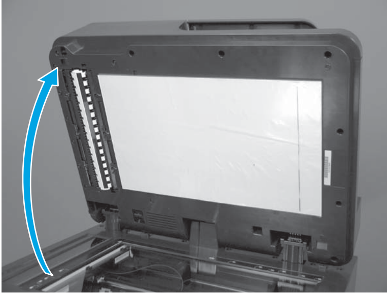
Figure 1-88 Install a replacement document feeder white backing (7 of 9)
