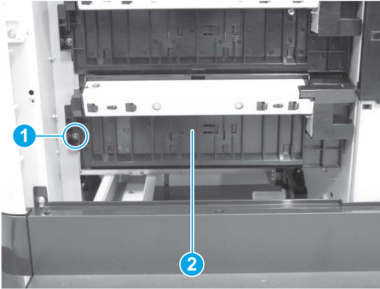
Figure 1-455 Remove the Tray 5 pickup assembly (2,500-sheet paper feeder HCI; 3 of 3)
