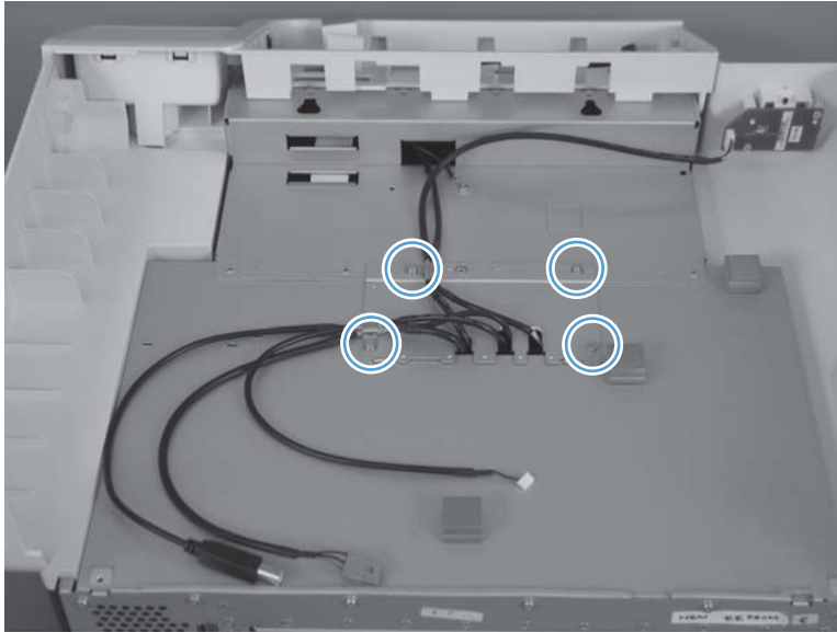
Figure 2-55 Remove the interconnect PCA, fan assembly, and DC connector PCA (1 of 6)
