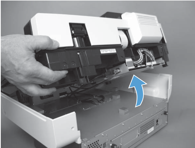
Figure 2-36 Remove the flatbed scanner and ADF assembly (6 of 7)
