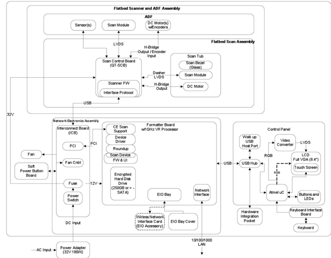
Figure 1-1 Hardware subassemblies
