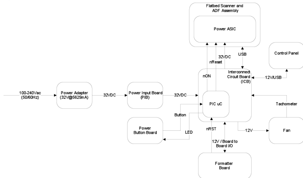
Figure 1-3 ICB connections
