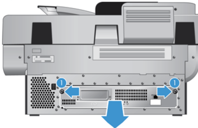
Figure 2-16 Remove the formatter (1 of 11)
