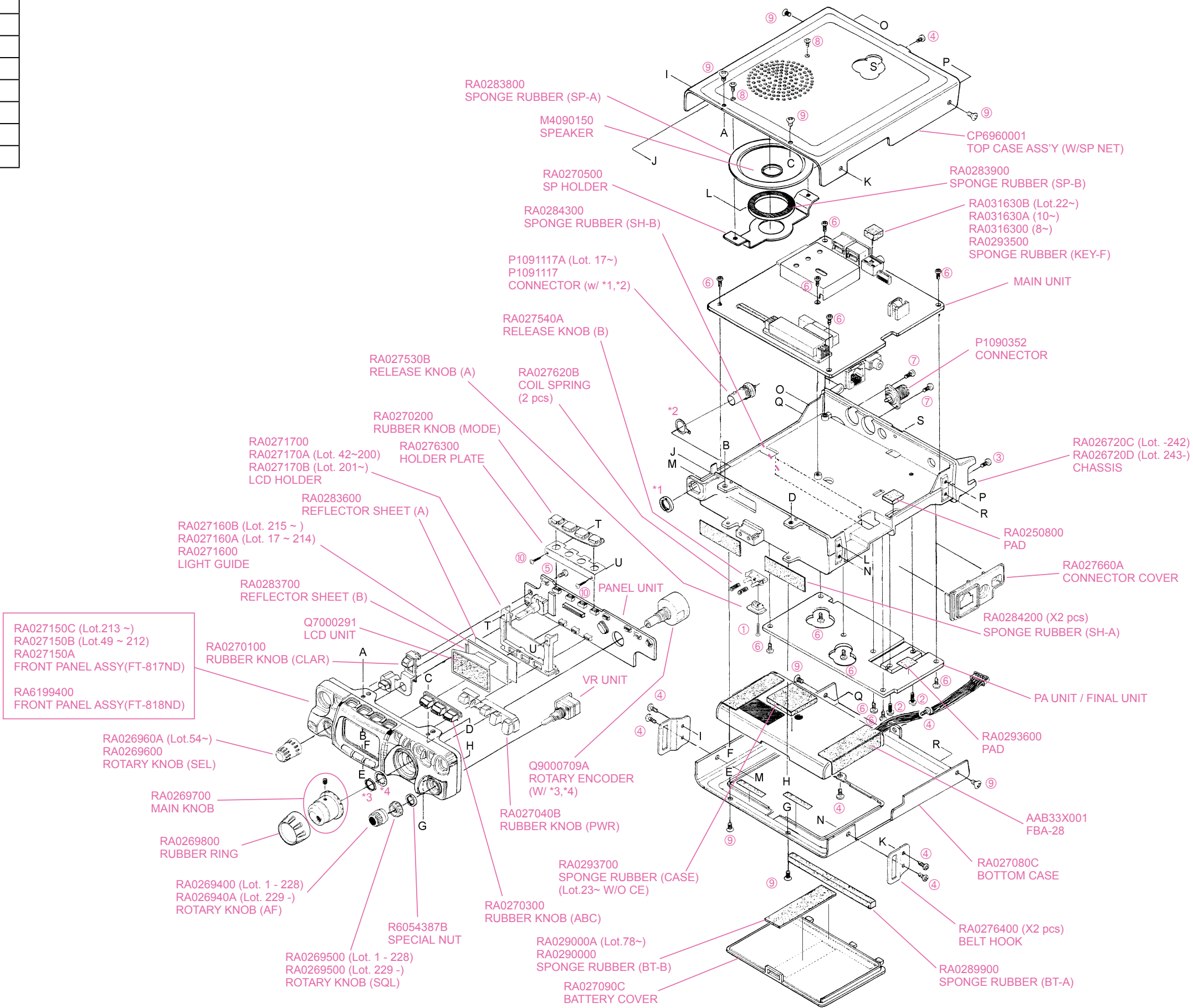
Exploded View-1
